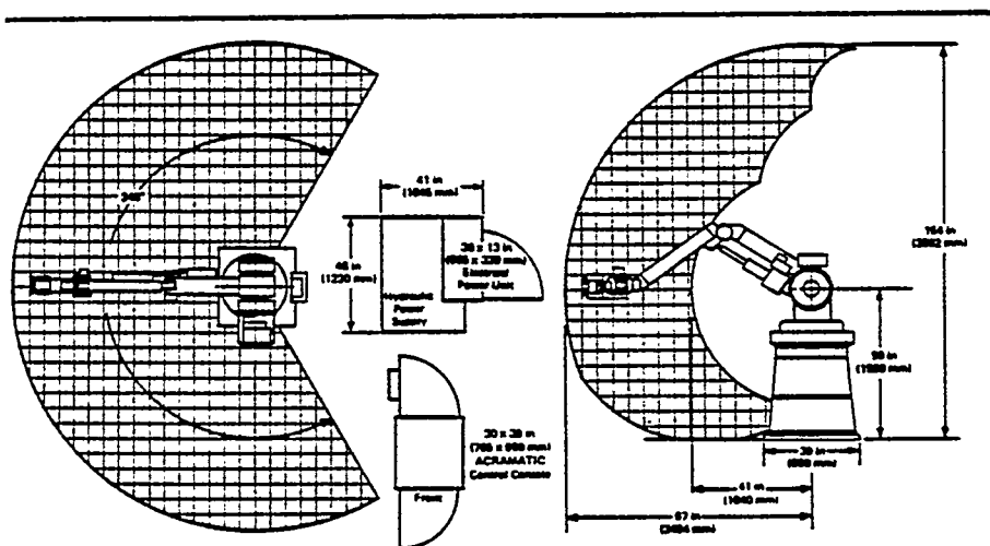
Basic range and floor space drawings
