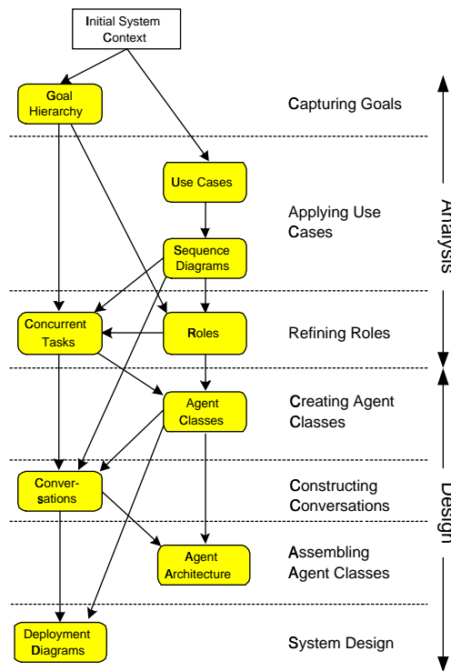
FIG. 4.1. MaSE Methodology
