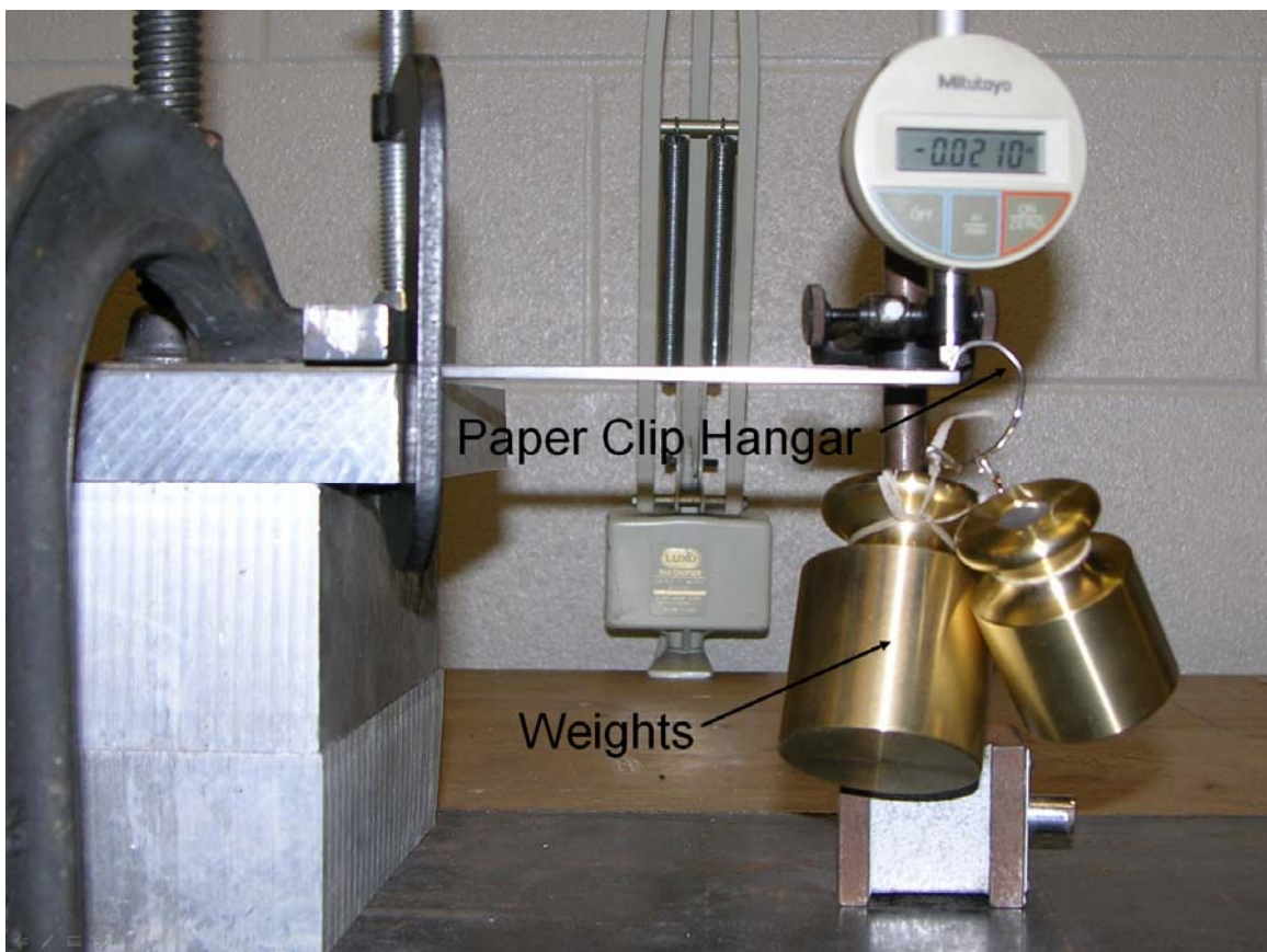
Figure 8. Cantilevered Beam with Weights Applied
