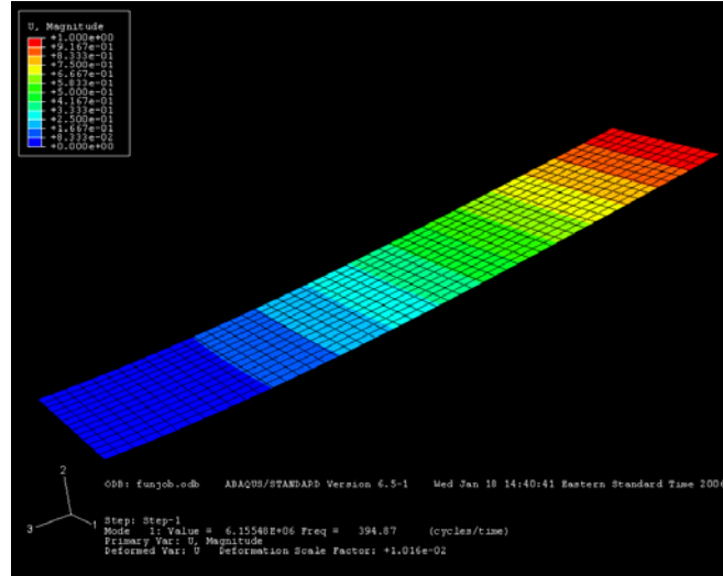
Figure 24. Plate Model
