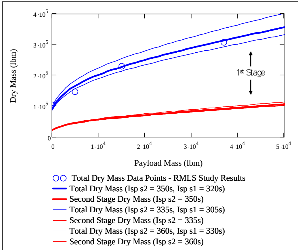
Figure 8. RLV Total Dry Mass versus Payload Correlated To RMLS Studies
