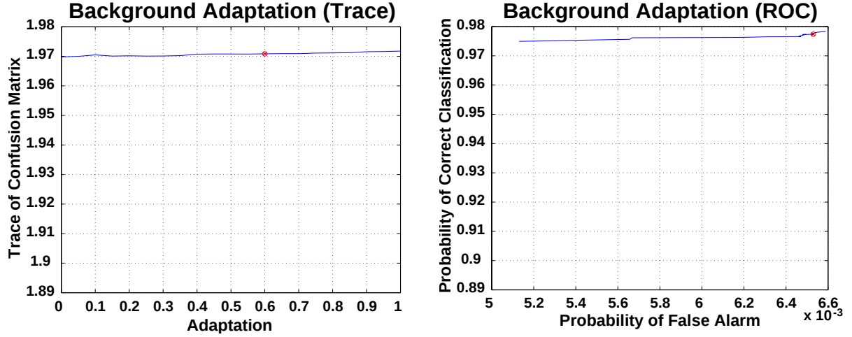
Figure 9: Performance as a function of the background histogram adaptation factor a_{bg} . The left graph plots the trace of the confusion matrix. The right graph shows the ROC curve. Graphs show the average performance over three 75 frame learning sequences. The optimal point is shown in red.
