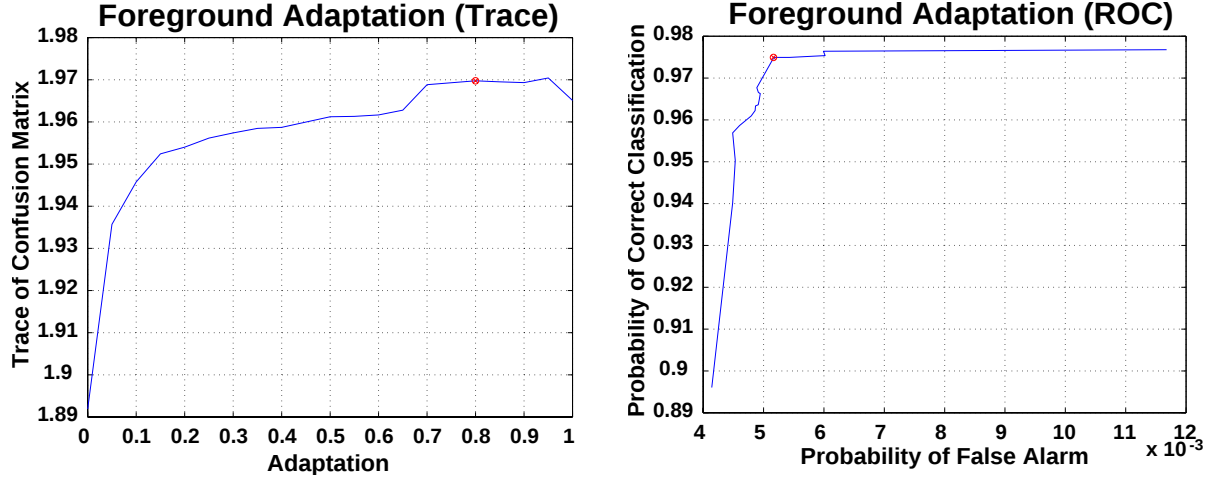
Figure 8: Performance as a function of the foreground histogram adaptation factor a_{fg} . The left graph plots the trace of the confusion matrix. The right graph shows the ROC curve. Graphs show the average performance over three 75 frame learning sequences. The optimal point is shown in red.
