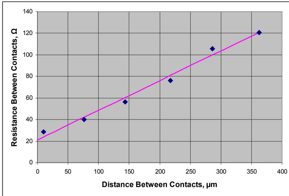
Figure 34. TLM data giving measured resistance between pads versus pad separation and the least squares fit line to the data (5-hour anneal at 1700^\circ\text{C} and 10^{-5} Torr).
