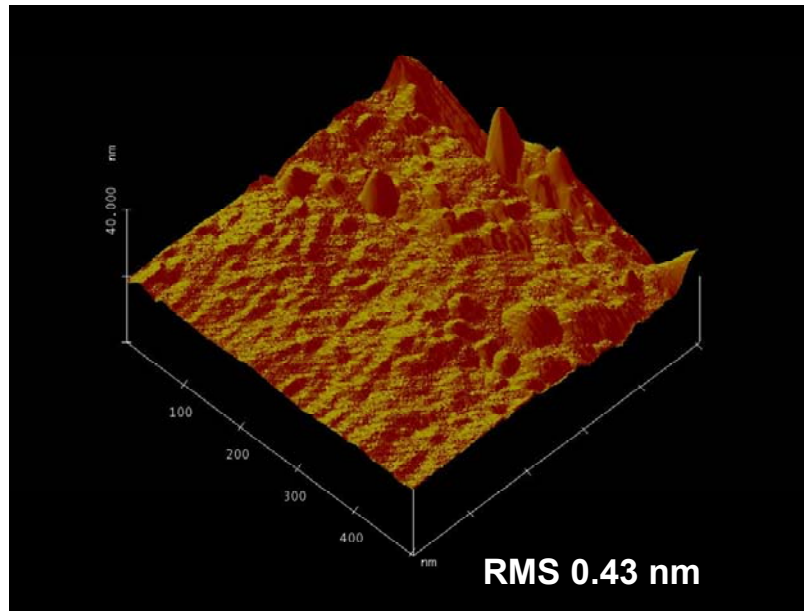
Figure 21. Atomic force microscopy image of the Si-face of the polished SiC wafer, showing typical scratch marks due to residual polishing damage.
