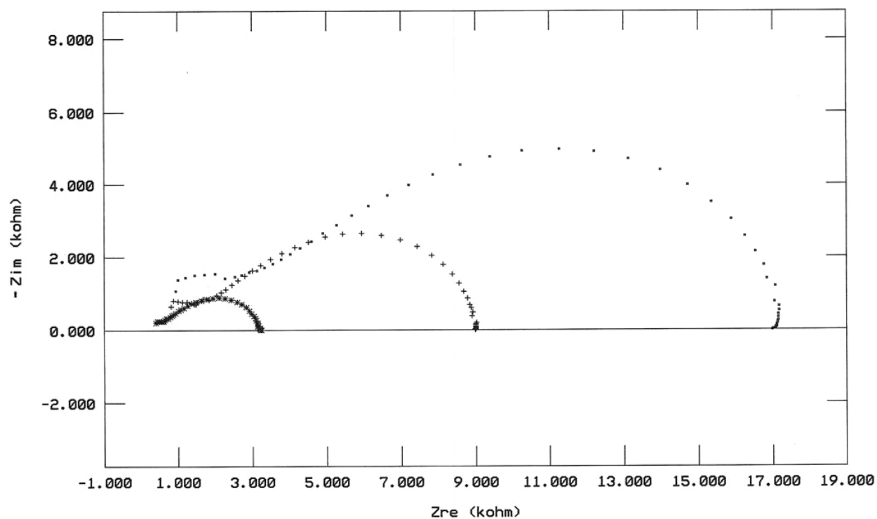
Figure 7. Nyquist plots of Cu/Li 2 Pc(Sol. Cast 20 \mu\text{m} film 4)/Cu cell at 21°C and pressures of 24,000 psi, 12,000 psi and 8,000 psi.
