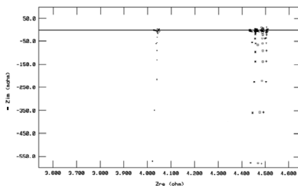
Fig. 9. Nyquist plots for thin film \text{Li}_2\text{Pc} cast onto carbon at (a) \blacksquare , 21°C, (b) + , 0°C, (c) * , -25°C and (d) \square , -50°C.
