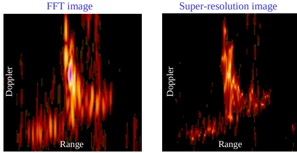
Figure 3 FFT vs. AR Doppler image.
