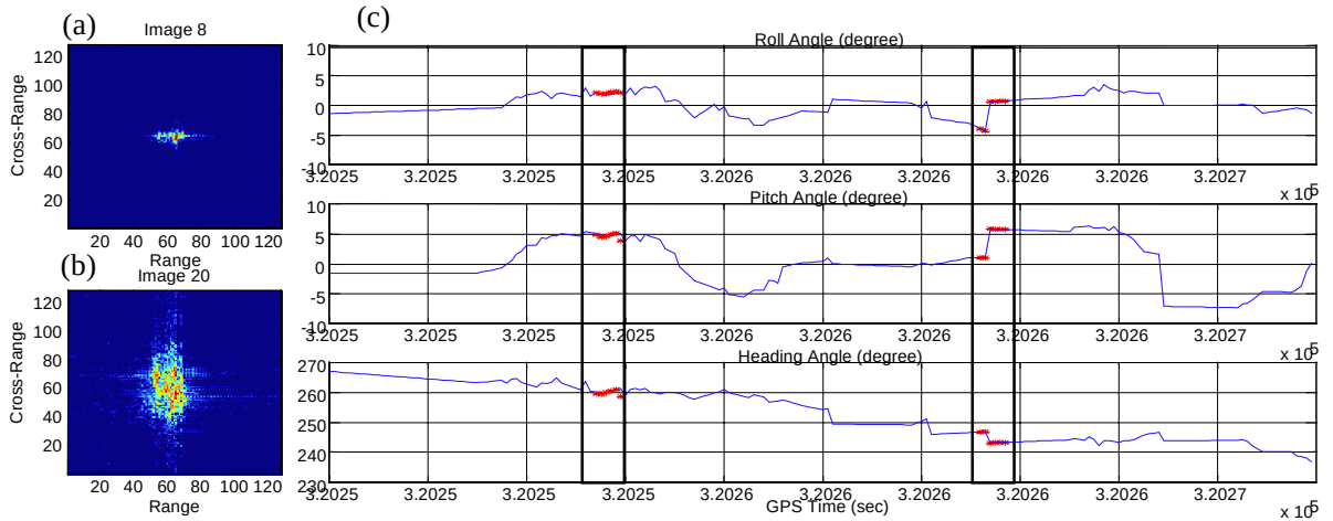
Figure 6. Effect of motion perturbation on ISAR images.
