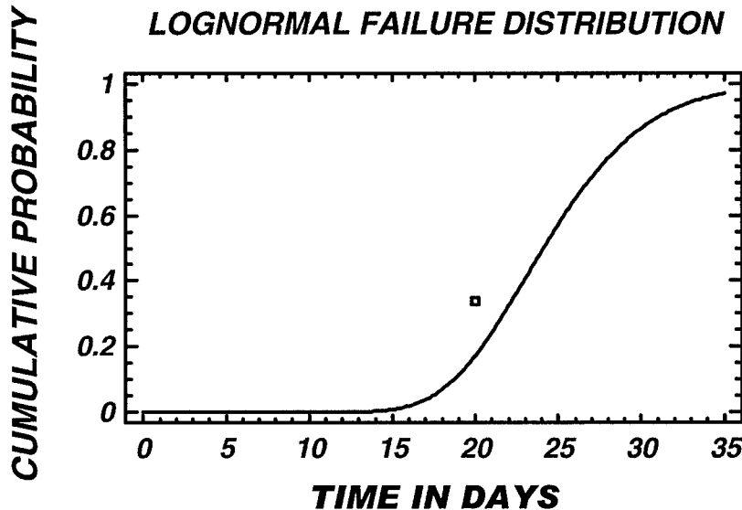
Figure A-3. Lognormal Failure Distribution for the Y109 Lot at 375°F
