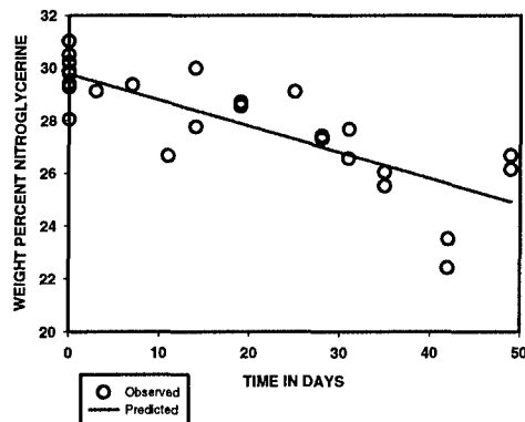
Figure A-2. Weight percent NG vs. time
