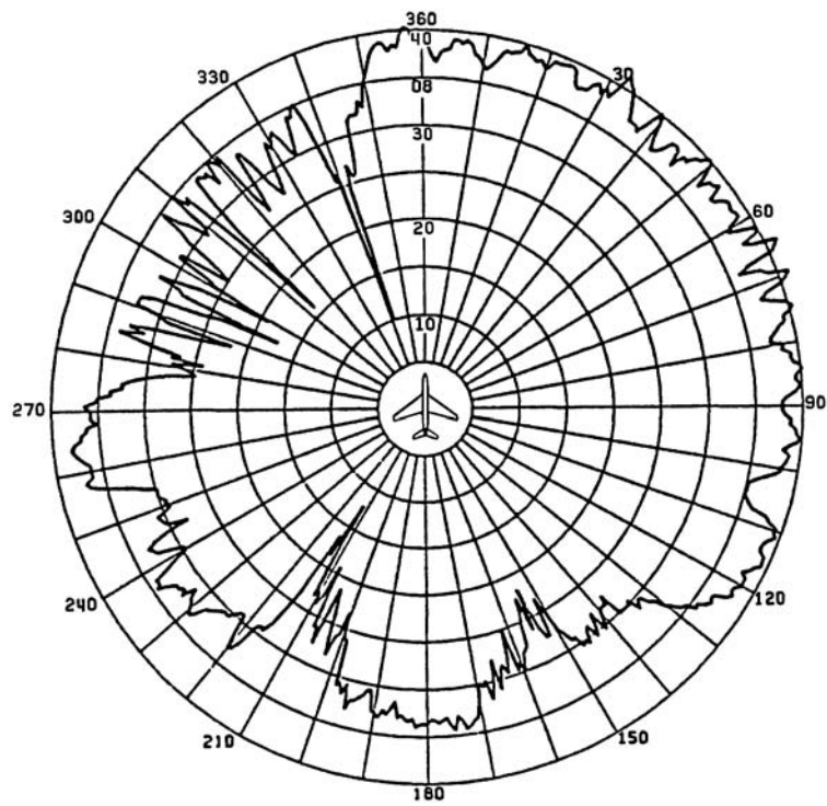
Figure 19B.B-3. Radiation Pattern of Telemetry Antenna, Trajectory Right-hand Circle, Bank Angle 15 Degrees, Frequency 2401 MHz.
