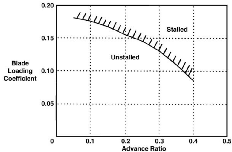
Figure 12A-1. Blade Stall Boundary.
