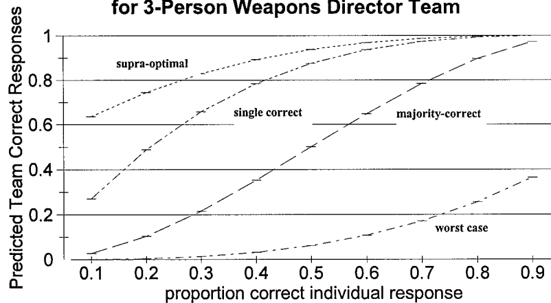
Predicted Proportion Correct Response for 3-Person Weapons Director Team
