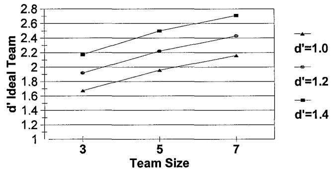
Team Size Influences on Ideal d' with Various Levels of Member d'
