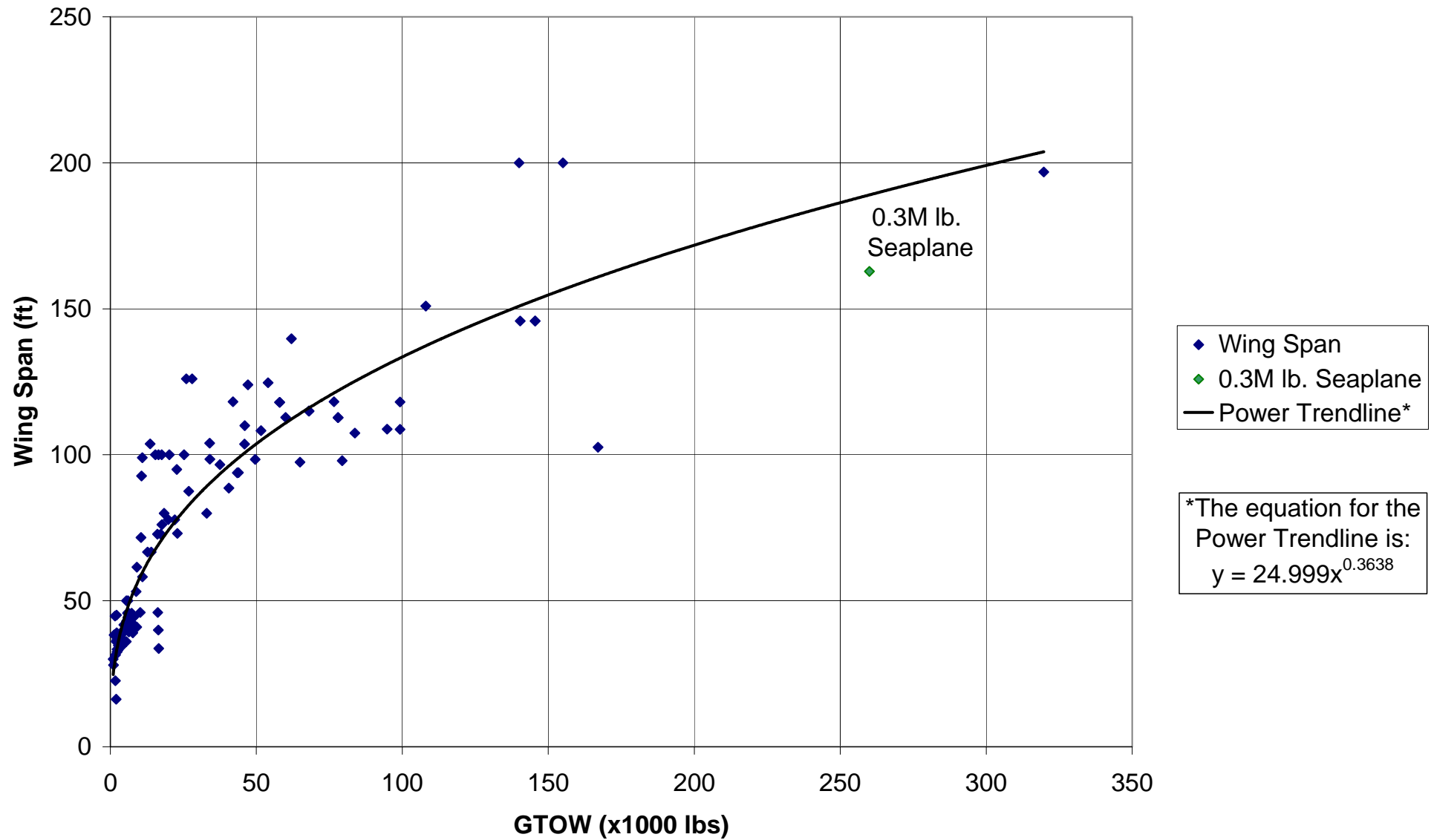
Figure 6. Seaplane parametric chart – Wing span vs. GTOW with 0.3 M lb. Seaplane.
