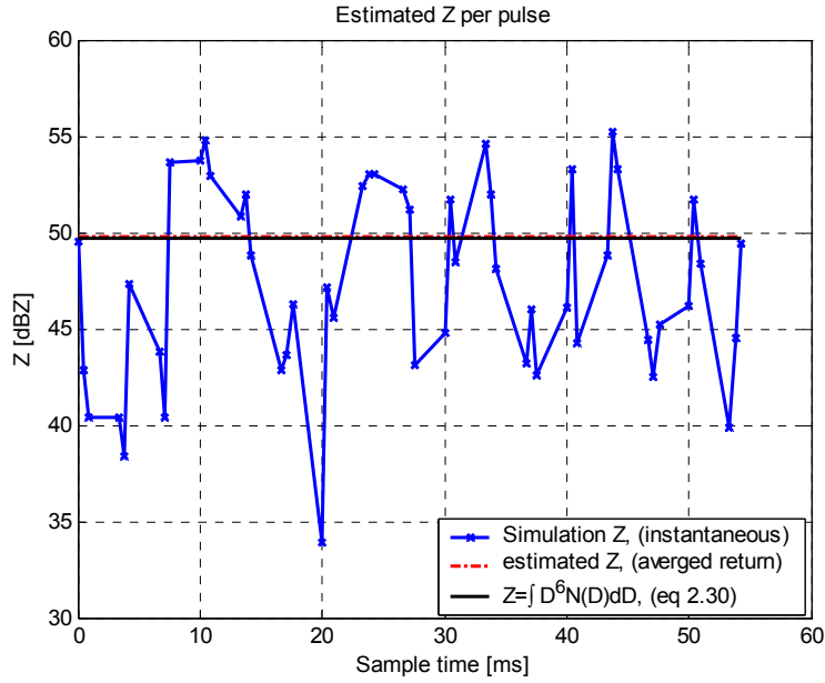
Figure 26. Temporal Sampling, Stepped Frequency. PRF_1 5000 Hz, PRF_2 300 Hz. Velocity Spread 2 m/s between pulses and within pulses for drops of different sizes.
