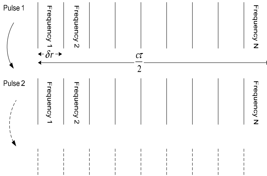
Figure 20. Pulse Compression implementation.
