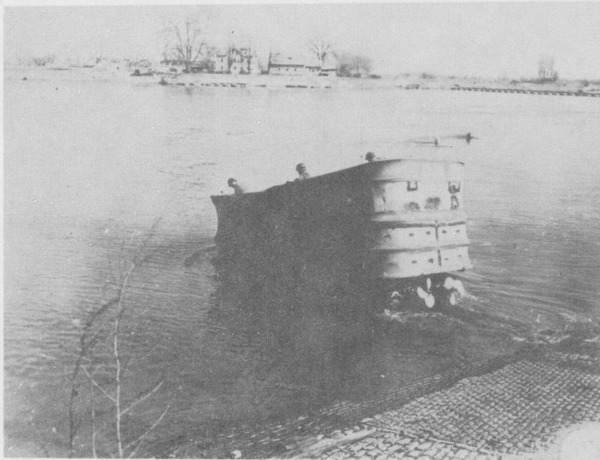
Photo No. 15 DD TANK ENTERS RHINE RIVER AT NIERSTEIN - (One that has already crossed is seen climbing on far shore. Bridge in background was uncompleted at this time).
