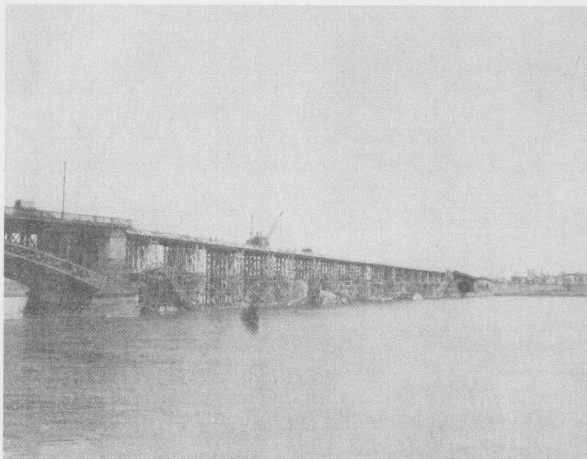
Photo No. 37 MILITARY FIXED BRIDGE UNDER CONSTRUCTION ON SITE OF DEMOLISHED HIGHWAY BRIDGE AT MAINZ.
