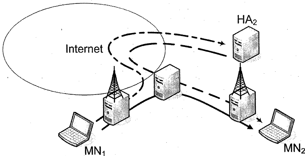
Abbildung 4.5: Das Triangular Routing Problem
