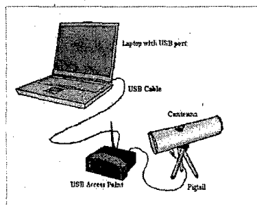
Abbildung 1.3: War Driving System [19]
