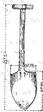
Fig. 4 U.S. Intrenching Shovel
