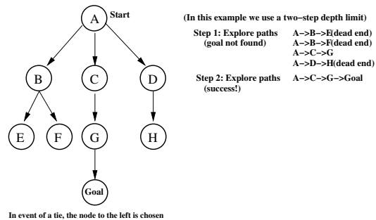
Figure 18: Iterative Deepening Search.
