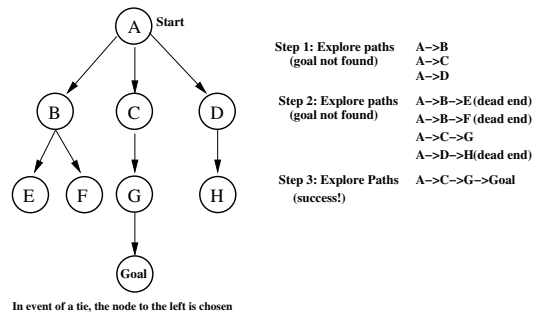
Figure 17: Breadth First Search.
