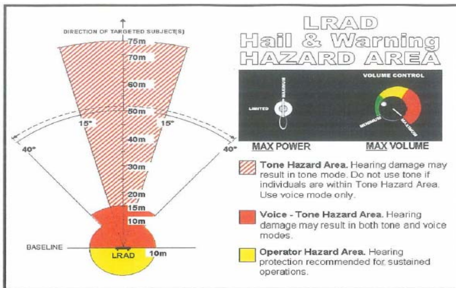
Figure 10. LRAD Beam Distribution
