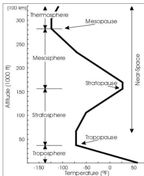
Figure 5. Temperature Profile through Near-Space. 143
