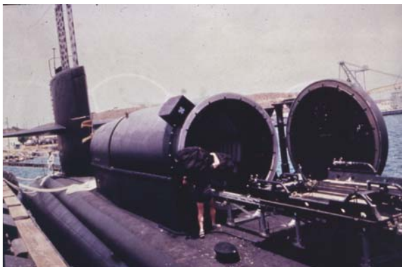
Fig. 37-12. (a) A Dry Deck Shelter (DDS) is being installed onto a host submarine. (b) US Navy SEAL (sea, air, land) divers launch a SEAL delivery vehicle (SDV) from the DDS. Photographs: Courtesy of US Special Operations Command, MacDill Air Force Base, Tampa, Fla.
