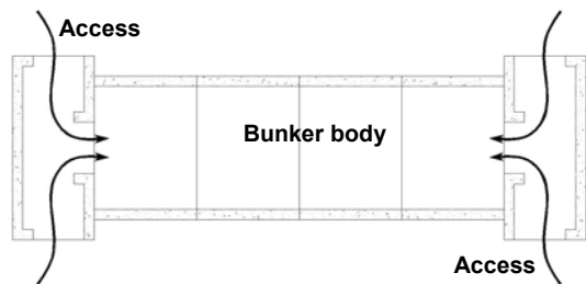
Figure 3. Entrance configuration of ERDC bunker
