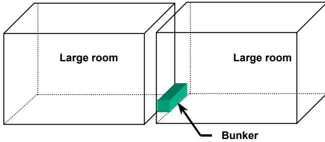
Figure 5. BLASTX model
