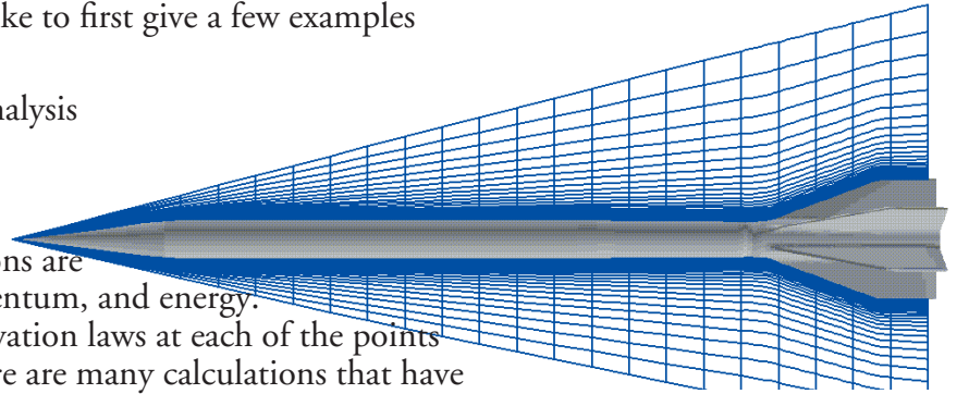
Computational grid.
