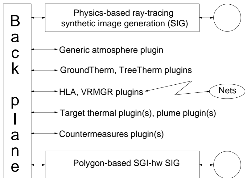
Software simulation back plane.
