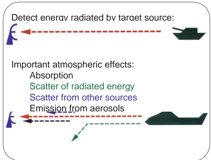
Energy transport: basic sensor scenario.
