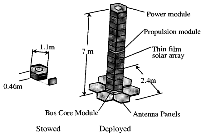
Figure 1 TechSat 21 Design
