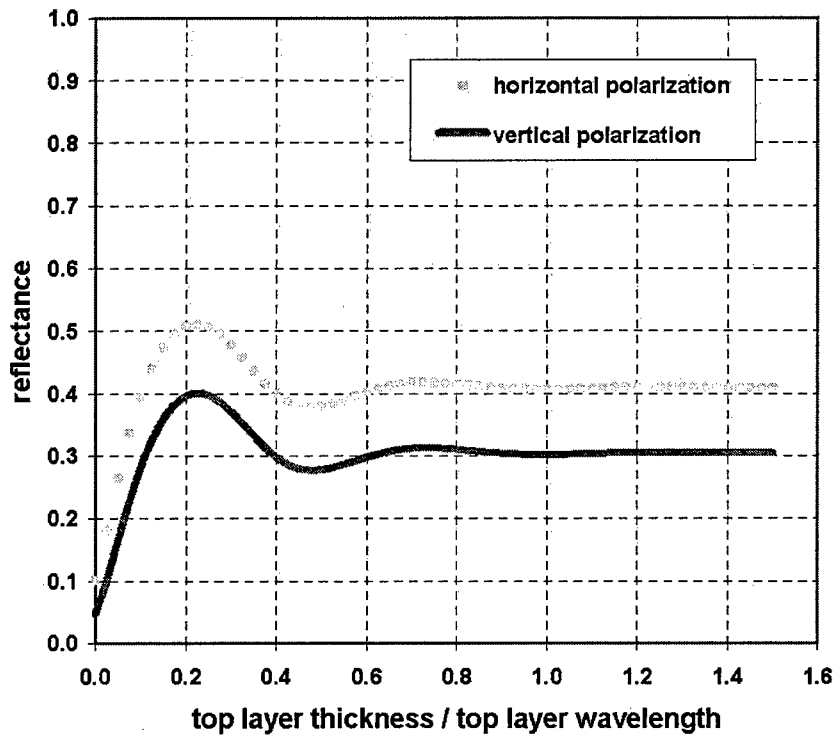
Figure 27. Reflectance from a high-loss moist layer at an incidence angle of 30 deg
