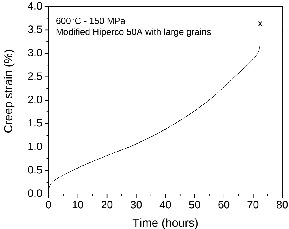
Figure 15. Creep strain versus time at 600°C and 150 MPa for a modified Hipercó 50A specimen with large grains.
