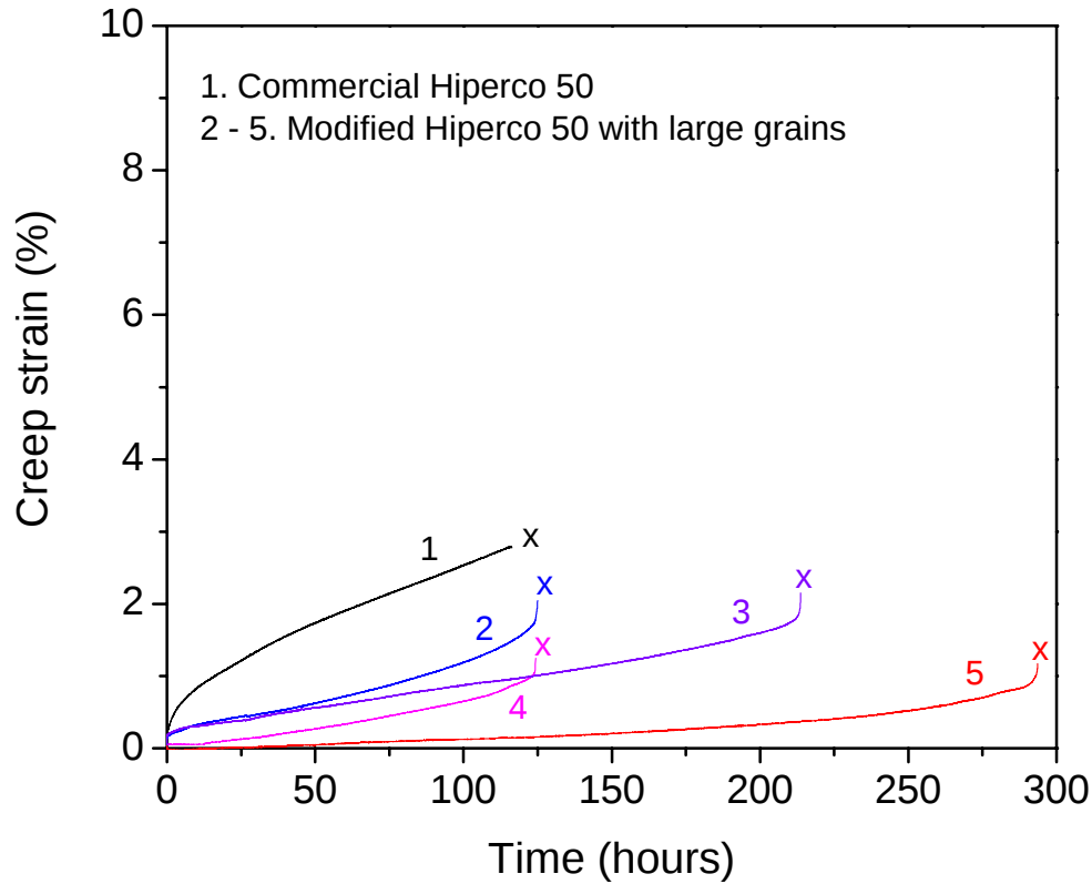
Figure 19. Creep strain vs. time for another set of commercial and modified Hipercro 50 specimens tested at 600°C under 150 MPa.
