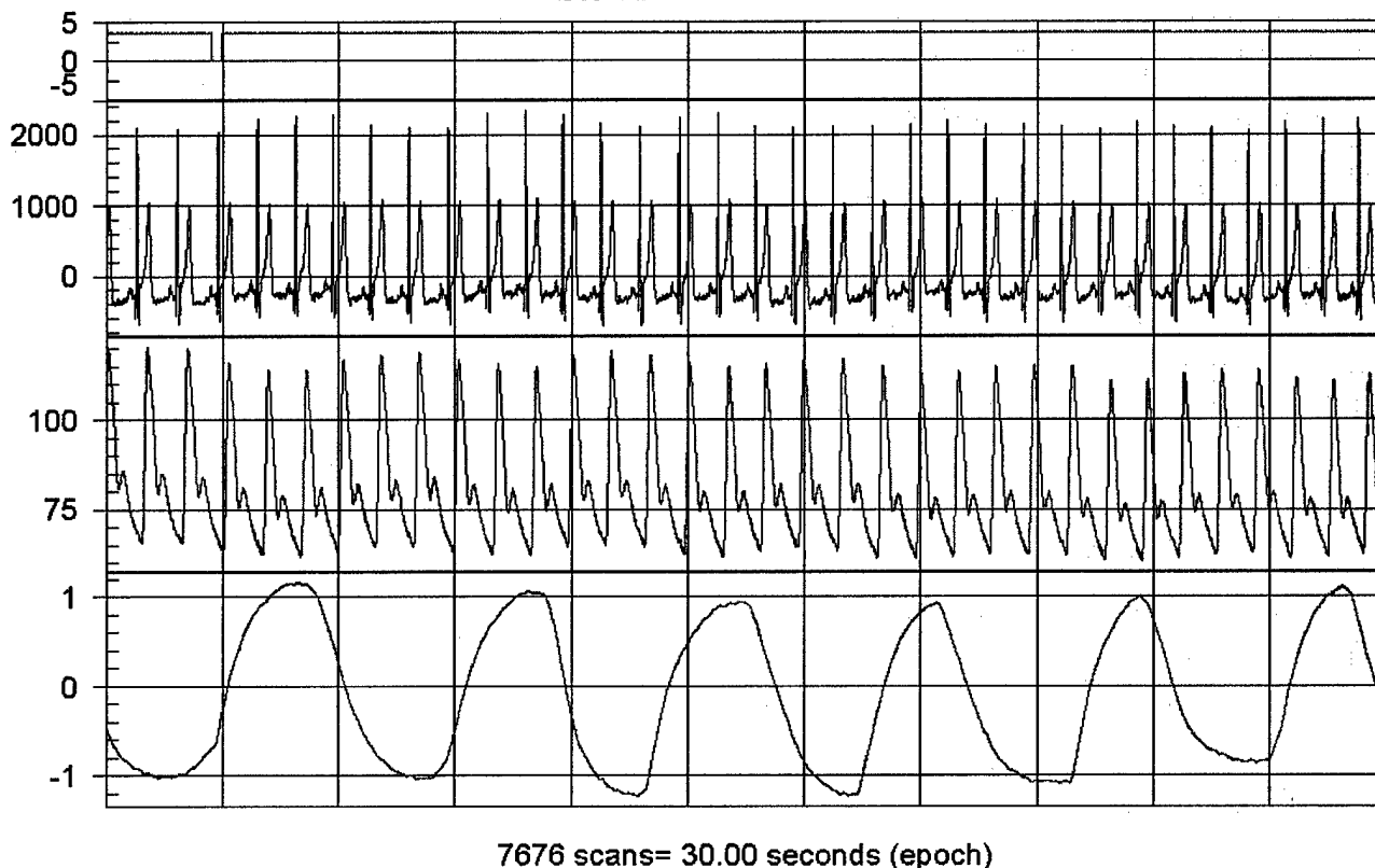
Figure 1 Representative 30-second record of ECG, radial artery tonometric BP and respiration during the first 5-minute baseline period. The screen code VV4136M is a unique identifier for data from this volunteer: Study VV, volunteer #4136, multichannel data sampled at 256 Hz. The upper scan number ranges identify these data from the beginning of the record. The vertical axes for the first (marker), second (ECG) and fourth (respiration) channels are in arbitrary units, the second channel (BP) is in mmHg. The marker channel, shown in green at the top of the figure, indicates the onset of a timed 5-minute baseline period as marked by the investigator.
