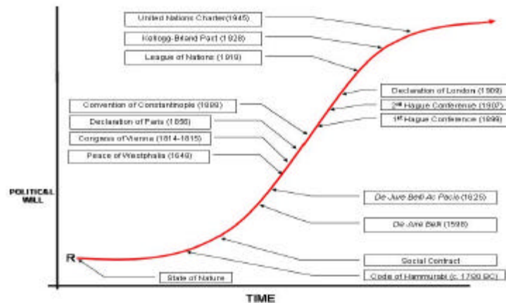
Figure 3. Time-Series Graph
