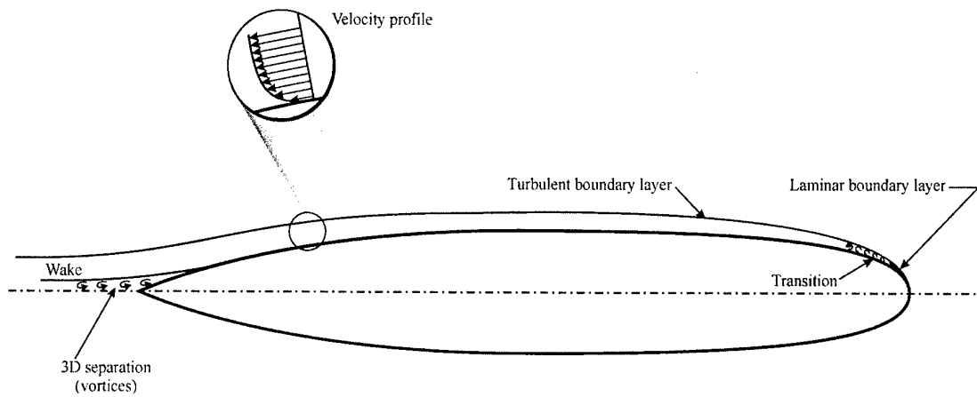
Figure 16. Flow around a submarine
