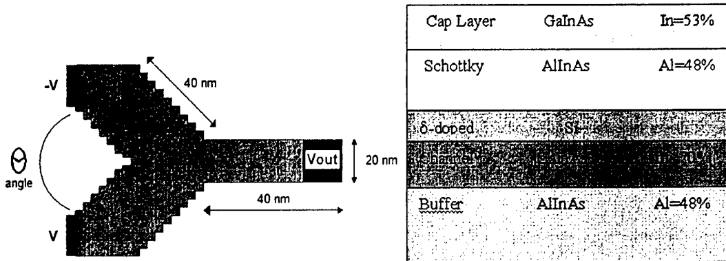
Figure 1: Representation of the simulated Y-Branch Junction(YBJ)
