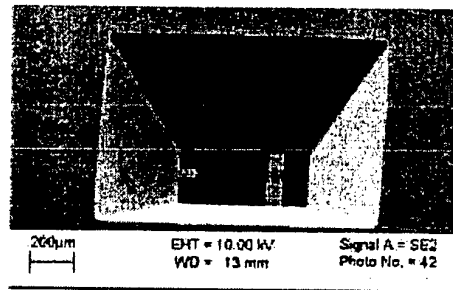
Fig 3. Back side view of the sensor window to allow liquid operation.
