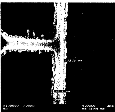
Figure 3 SEM of T-branch using wet etching process
