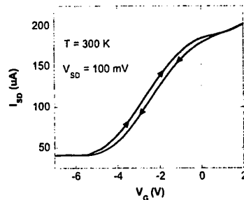
FIG. 4: Memory effect shown by the clear hysteresis in the I_{SD} vs V_G curve, which was obtained at a fixed V_{SD} = 100 \text{ mV} and measured at room temperature.
