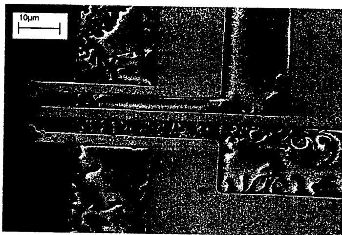
Figure 3. By applying voltage between the lower two electrodes we can preferentially assemble the nanotubes between them. The tubes in the remaining regions can be seen assembling there during the evaporation of the solution.
