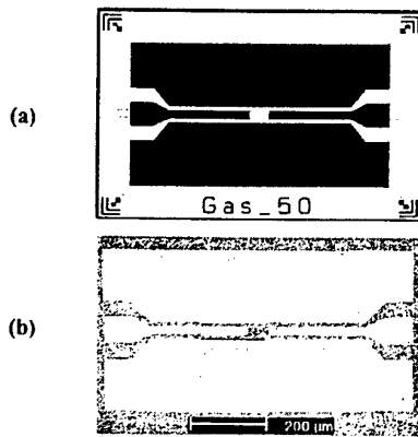
Fig. 1: (a) Lithographic mask and (b) realization of a simple ballistic channel, embedded in CPW accesses. In Fig. 1(a), dark area is metal and white area is 2DEG channel of length 60 μm and width 26 μm.
