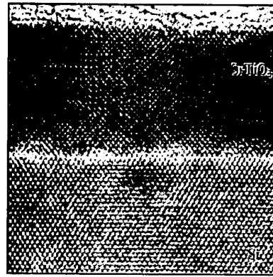
Figure 2: HRTEM picture of a SrTiO 3 - silicon interface
