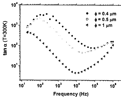
Fig. 3.: Dielectric loss tangent at 300 K.
