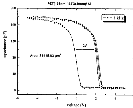
Figure 4: C-V curve of a Pt/PZT/STO/Si MFIS diode at f=1kHz.
