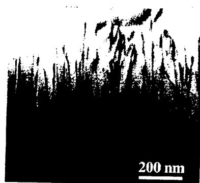
Fig. 1 TEM micrographs of InGaAs ( \times\sim 30\% ) structure on GaAs substrates
