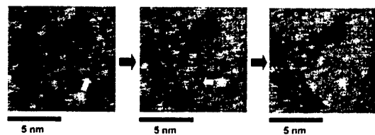
Fig. 3. Series of time-lapse STM images ( 10 \times 10 \text{ nm}^2 ) of (a) BMT and (b) BPMT. Each image was recorded under a constant condition with a sample bias of +1.0 V and a tunneling current of 30 pA at room temperature. Some isolated molecules move in the directions indicated by arrows in the BCO SAM matrix.
