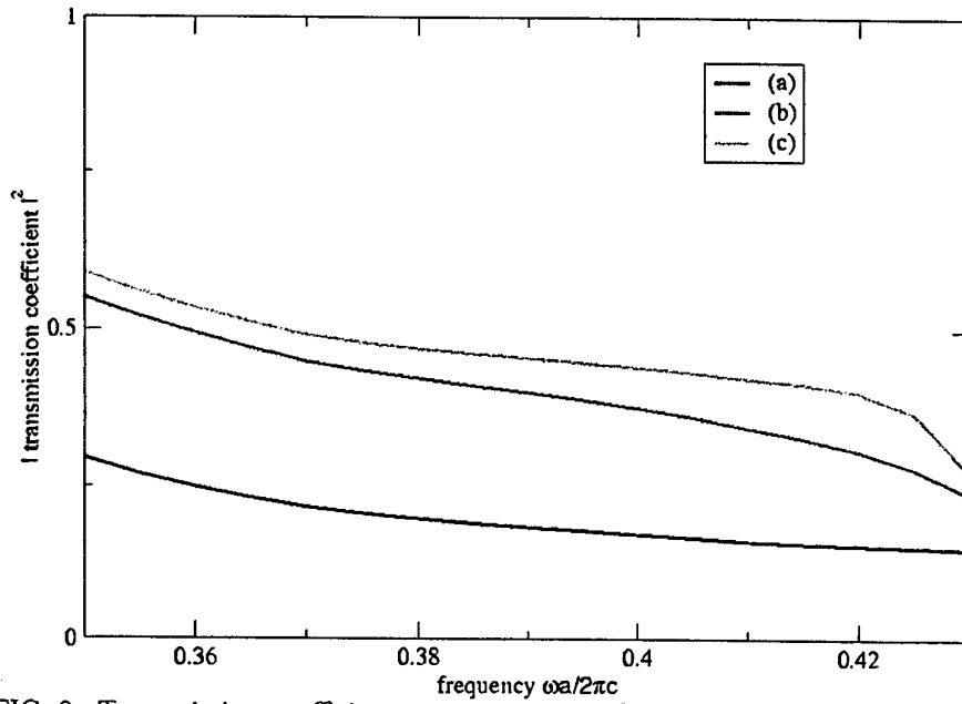
FIG. 2. Transmission coefficient corresponding to the structures shown in Fig.1 when only the guided mode with the largest |\bar{k}| in propagation direction is excited in the incoming field from the left ( I_m^L = \delta_{m1} ) and there is no incoming wave from the right ( I^R \equiv 0 )
