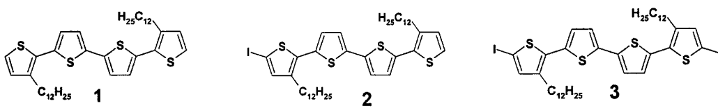
Figure 1 Chemical Structures of oligothiophene derivatives investigated
