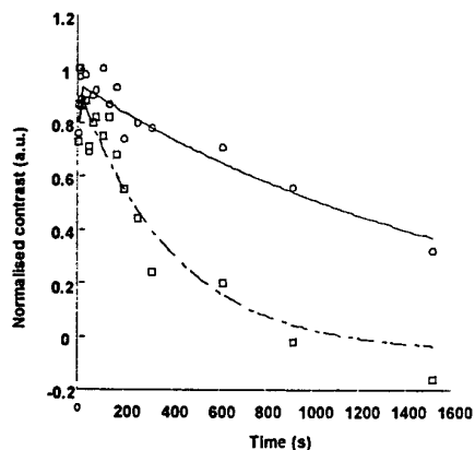
Figure 1: Leakage of chlorin e_6 -loaded nanoparticles (-O-) as compared to free dye -□-) as measured by means of fluorescence contrast in the CAM model.
