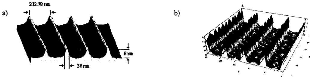
Figure 2. A comparison between experimental and simulation results: a) one-dimensional array of Cr features obtained by laser focused atomic deposition (NIST Electron Physics Group) b) simulated surface obtained using one-dimensional standing wave field and limited diffusion model
