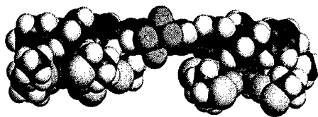
Figure 2: "Paddle Wheel" rotor with rotating in green.
