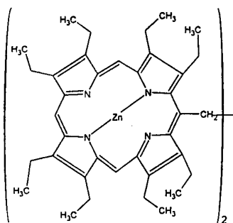
Figure 1. Bis-zinc ethane-bridged porphyrin dimer (1) molecular structure
