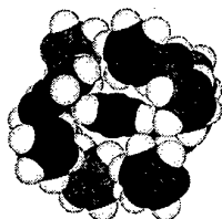
Figure 1: Fluorobenzene rotor group (red) Surrounded by neighboring triphenyl groups (blue)
