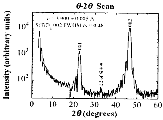
Figure 1: XRD pattern of a SrTiO 3 thin film deposited on Si (100)
