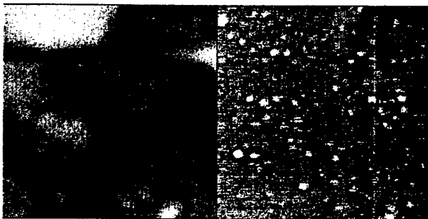
Fig. 3. AFM tapping mode image of a thiopropylsilanized GaAs substrate with silver colloids deposited onto it (Height contrast – left, Phase contrast – right). 250nmx250nm area. Maximum height scale is 10nm.
