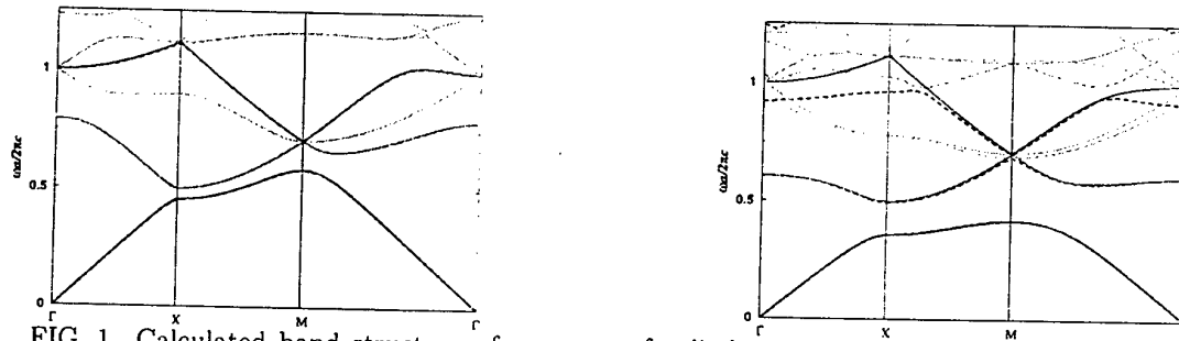
FIG. 1. Calculated band structure of an array of cylinders of Silicon ( \epsilon = 11.9 ) in air, with radius (in units of the lattice constant) r/a=0.05 (left) and r/a=0.1 (right). Continuous lines are the results of the method presented here and dashed lines are the result of a multigrid technique depicted for comparison. These plots show that the method is exact for moderate radii and slightly deviates when bands well above the first bandgap are considered.
