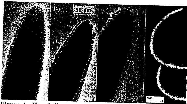
Figure 1: The shell structure of the deposited tips. (A) This structure consisting of gold particles embedded in amorphous carbon was observed for depositions in N_2 , 80%Ar/20% O_2 , and 60%He/40% H_2 . (B) In tips deposited in water vapor pressures above 0.5 Torr, a gold core was found. The core is surrounded by a crust of material similar to the material in A. (C) Contamination layers can be seen surrounding the crust. (D) SEM image showing the extreme bending of originally straight tips with contamination layers, after subsequent exposure to electron radiation.
