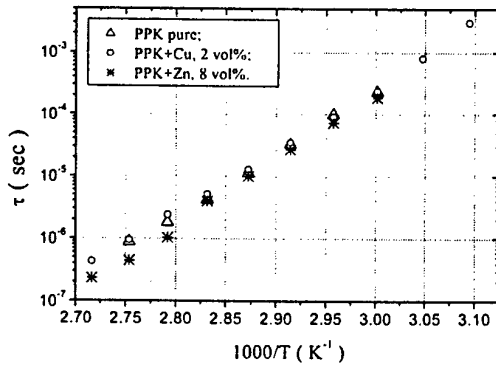
Figure 2. Temperature dependencies of the characteristic relaxation times of the \alpha -process for samples pure PPX ( \Delta ), PPX+Cu, 2vol% ( \circ ), and PPX+Zn, 8vol% ( \ast ).
