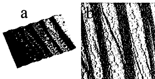
Fig. 4. (a) 0.3 ML Co evaporation on the striped structure of Fig. 1. Co sticks preferentially to steps and Ag stripe edges in Cu terraces (100nm). (b) The same surface after 0.8 ML of Ag and 2.2 ML of Co. The faceted structure and the contrast of Fig. 1 is maintained, suggesting the presence of alternating stripes with different Co content (200nm, image derivative along the horizontal direction).
