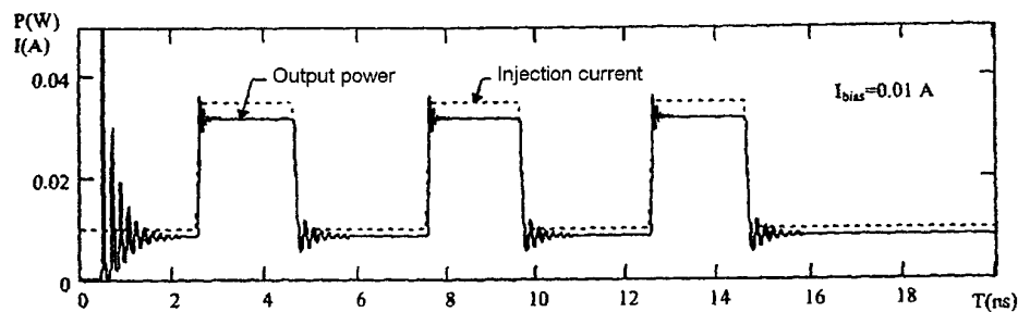
Fig. 1. Output power and injection current versus time when the QW laser is excited with a train of pulses
