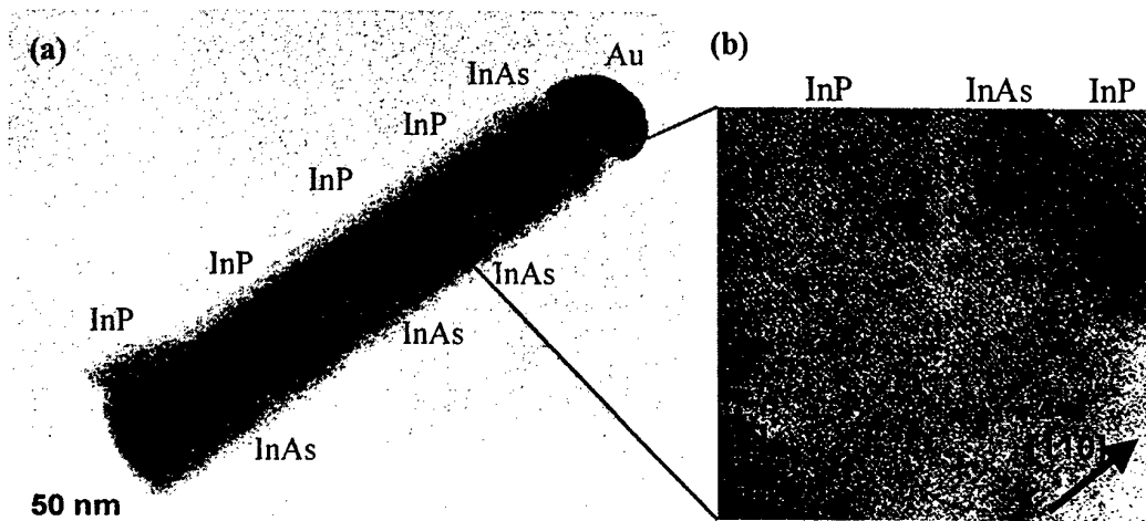
Fig. 1. InP/InAs/ InP one dimensional heterostructure. (a) TEM image of the one dimensional heterostructure, showing the contrast between the InP layers (grey) and InAs layers (dark). (b) High resolution TEM image of one section of the heterostructure.
