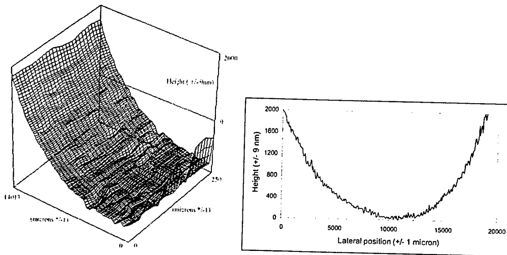
Figure 2. On the left the microtopography of a 250 \mu m slice of a 20 mm large WO film. On the right a profile of another zone of the tungsten film. A calculated stress of about 454 MPa was obtained.
