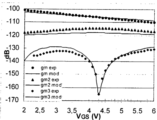
Figure 1. Measured (exp) and modelled (mod) values of ( g_{m1} ), ( g_{m2} ) and ( g_{m3} ), versus V_{GS} for n-type transistor at V_{SB} = 0V using equation (4).
