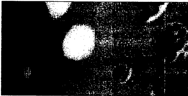
Fig. 2. AFM tapping mode image of a thiopropylsilanized mica substrate with silver colloids deposited onto it (Height contrast – left, Phase contrast – right). 122nmx122nm area. Maximum height scale is 5nm.
