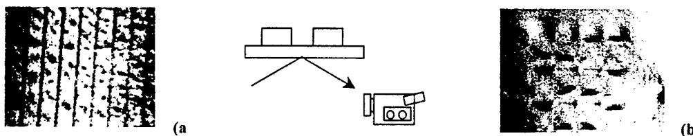
Fig. 3 Domain structure at the flat side of two structures with different patterns at selected field values: a) A continuous Co layer with a 1D pattern of Co stripes deposited at the opposite side and. b) A continuous Fe layer with a 2D square pattern deposited at the opposite side. The images size is around 600x450 \mu\text{m} .
