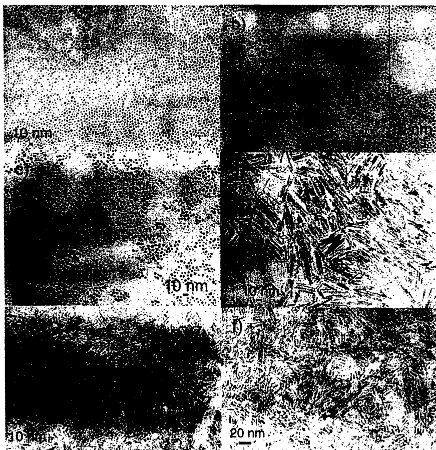
Figure 1. Some TEM micrographs of different ZnO amine capped nanostructures obtained from the oxidation of the organometallic precursor [ZnCy_2] : a) very slow oxidation (2 weeks) in Tetrahydrofuran (THF) as solvent with 1 equivalent of Hexadecylamine (HDA) as stabilizing amine. b) oxidation in Heptane as solvent with 1 equivalent of HDA as ligand. c) oxidation in THF with 1 equivalent of Octylamine (OA) as ligand. d) oxidation without solvent using 2 equivalents of OA as stabilizing ligand. e) oxidation without solvent using 2 equivalents of Dodecylamine (DDA) as ligand. f) oxidation without solvent using 1 equivalent of HDA as ligand.
