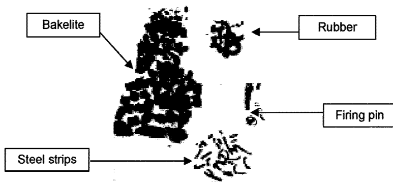
Figure 15. Fragments recovered from in-soil test after sifting sand and blast chamber debris.
