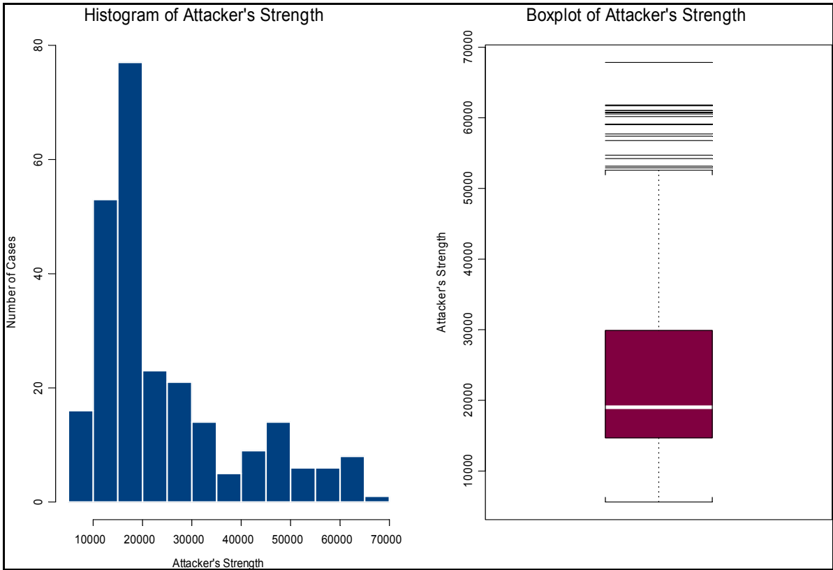
Figure 4. Explanatory Plots of Attacker's Strength
