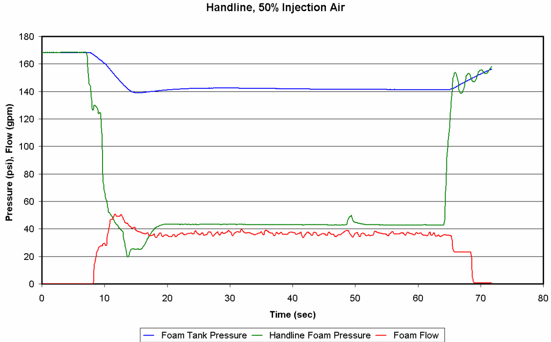
Figure 3. Handline Foam Flow and Pressure Data, 50% Air Injection.
