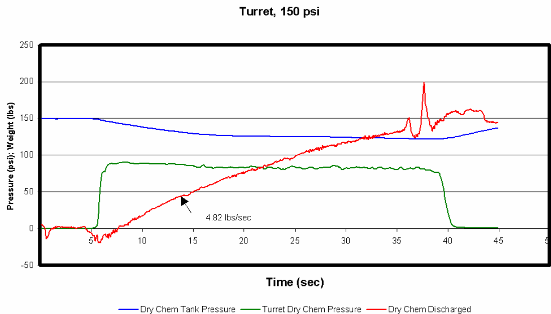
Figure 13. Turret Dry Chemical Flow and Pressure Data, 150 psi.
