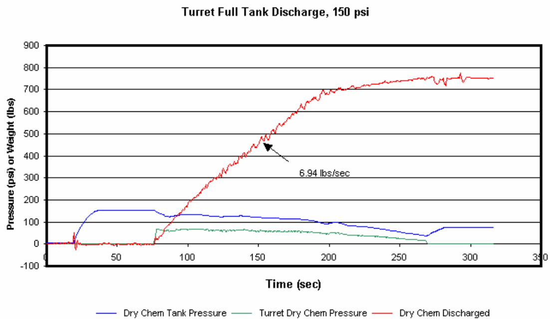
Figure 9. Full Tank Dry Chemical Discharge Using the Turret at 150 psi.
