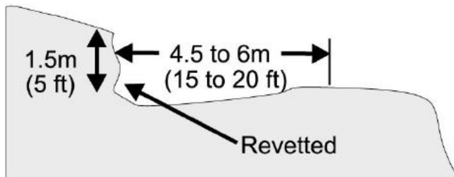
SIDEHILL CUT DITCH
