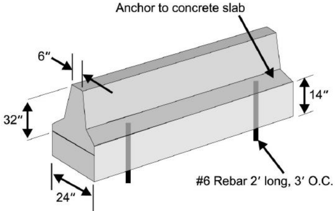
Figure 67. Jersey Barrier.
