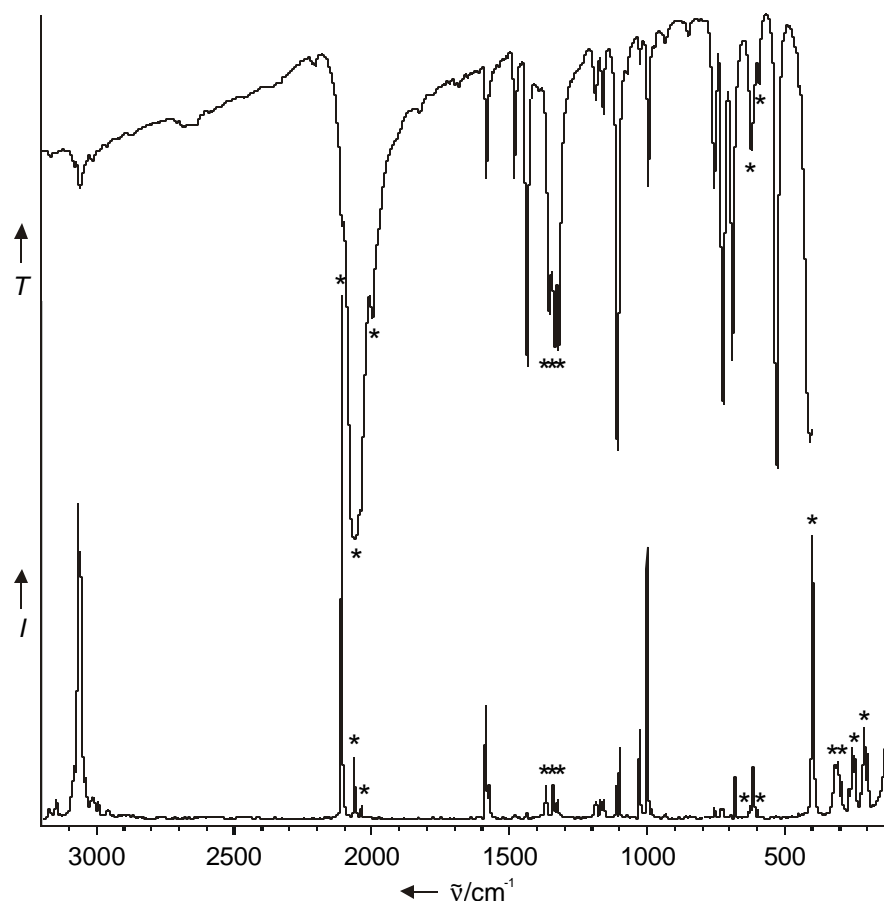
Figure 5. IR and Raman spectra of [\text{P}(\text{C}_6\text{H}_5)_4]_2[\text{Ti}(\text{N}_3)_6] . The bands belonging to the [\text{Ti}(\text{N}_3)_6]^{2-} anion are marked with asterisks.
