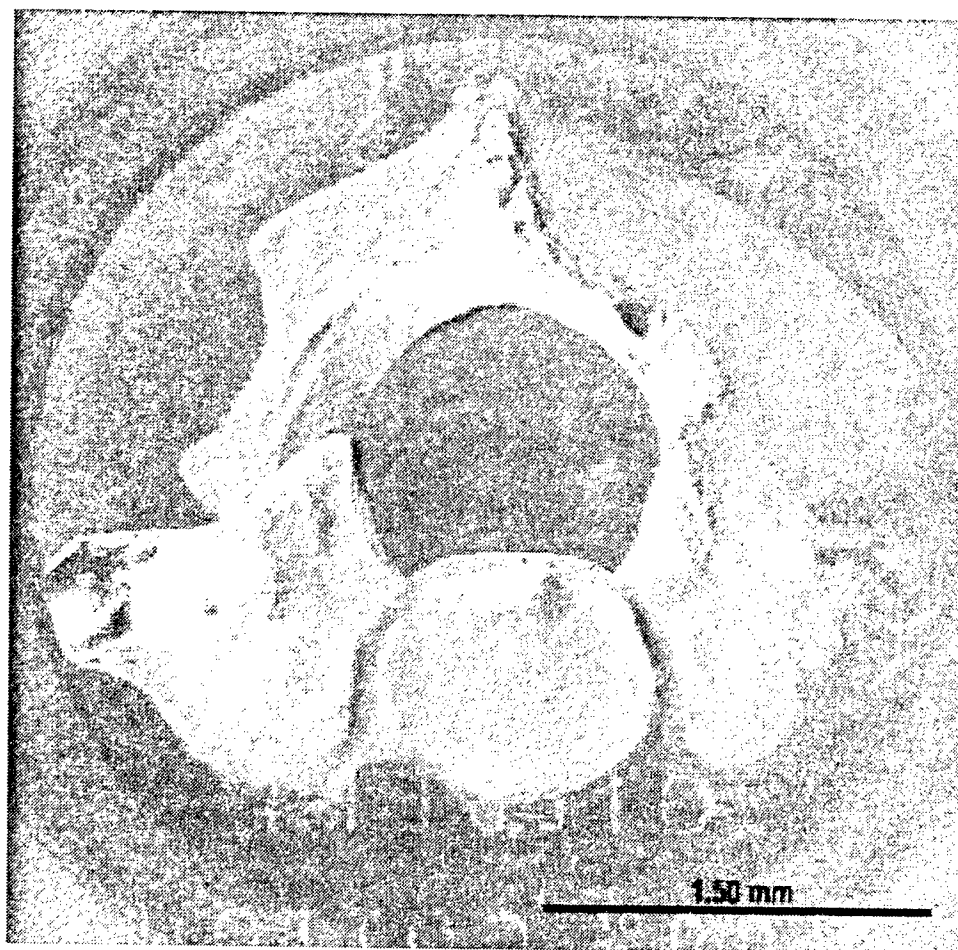
Figure 9. Scanning electron micrograph of a colubrid snake vertebra (LSUMG 4478) in anterior view.
