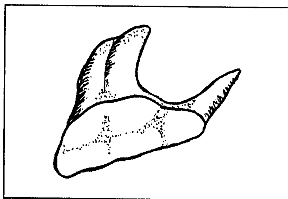
Figure 25. Example of fused/connected roots; in this case the lingual roots are strongly connected in sample number 10639.
