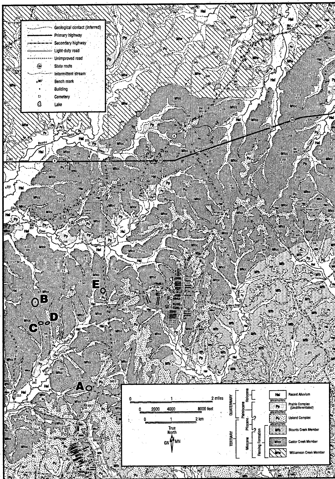
Figure 3. Main Miocene vertebrate sites within Fort Polk superimposed on a geologic map, after Schiebout and Ting (2001). Modified from Hinds (1999). A. DISC Site cluster; B. TVOR Site and sites N of it; C. TVOR S; D. TVOR SE; E. Shamrock.
