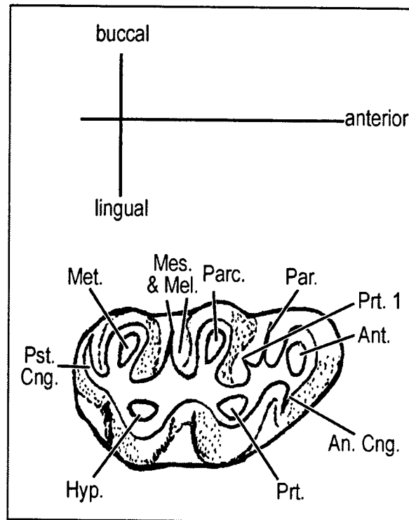
Figure 20A. Copemys M1 dental terminology: An.Cng. = Anterior Cingulum, Prt. = Protocone, Hyp. = Hypocone, Pst.Cng. = Posterior Cingulum, Met. = Metacone, Mes. = Mesostyle, Mel. = Mesoloph, Parc. = Paracone, Prt.1. = Protolophule I, Par. = Paralophule, Ant. = Anterocone. Sketch is of M1 of LSUMG 9207.
