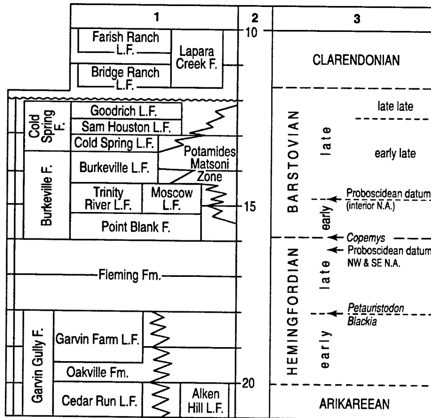
Figure 2. Fleming Formation vertebrate faunas in East Texas (1), age in millions of years (2), and North American Land Mammal Ages with selected defining taxa relevant to the Fort Polk Miocene Sites (3), after Schiebout and Ting (2001). Illustration after Schiebout and Ting (2001). Shaded area indicates intertonguing marine deposit. 1 and 2 modified from Schiebout (1994), which was modified from Tedford et al. , (1987, Fig. 6.2), 3 modified from Woodburne and Swisher (1995). After Schiebout and Ting (2001).
