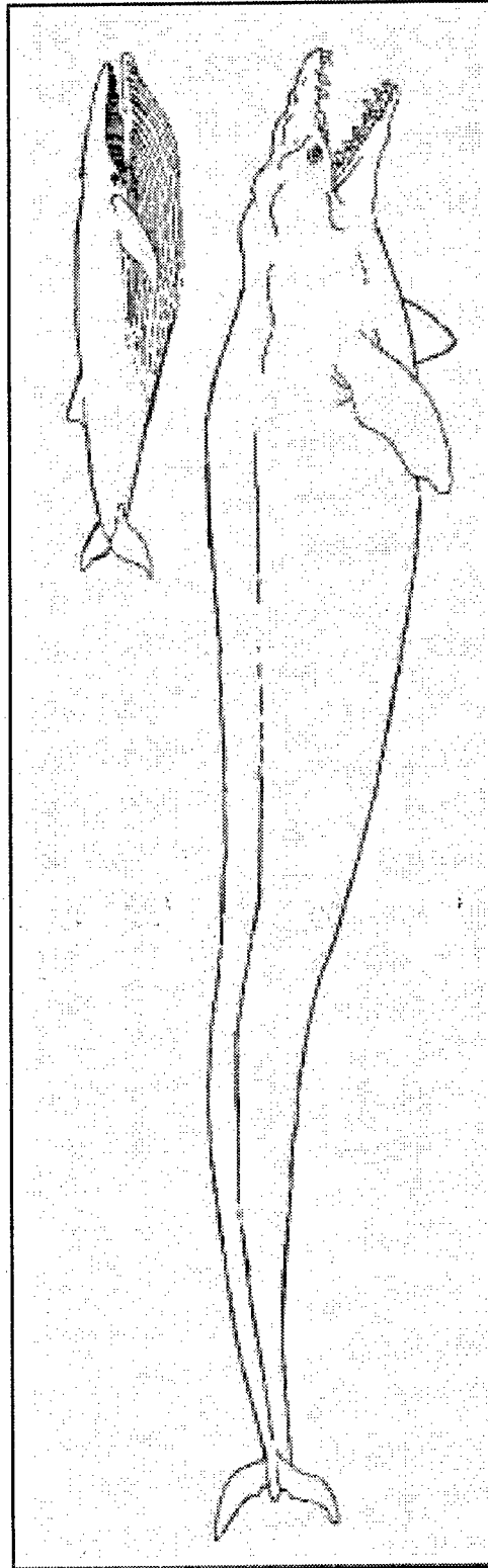
Figure 12. Sketch of a small baleen whale approximately the size of the one represented from Fort Polk by petrosals, compared to the larger Eocene Basilosaurus from Montgomery Landing, Louisiana.
