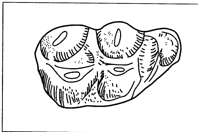
Figure 20B. Sketch of M1 LSUMG 9207.
