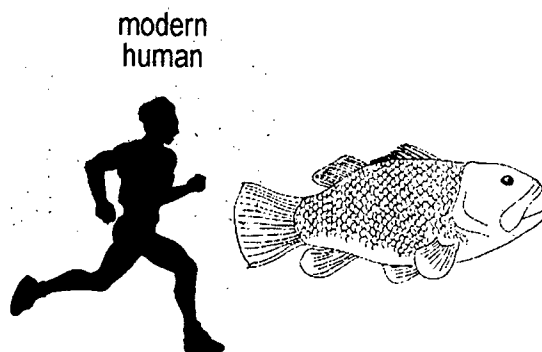
Figure 32. Sketch of giant sea bass in relation to a modern human.
