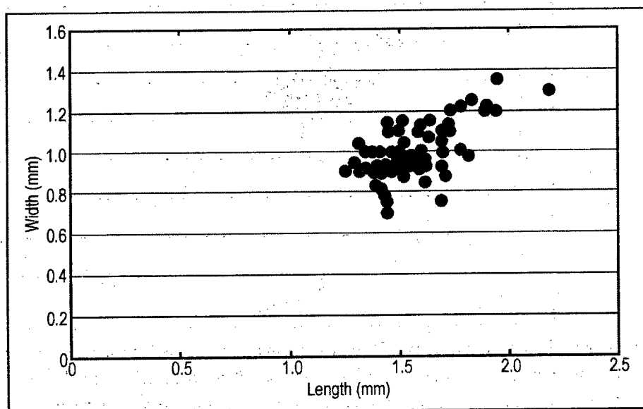
Figure 22. Distribution of Upper M1 samples for the Stonehenge site using width versus length.
