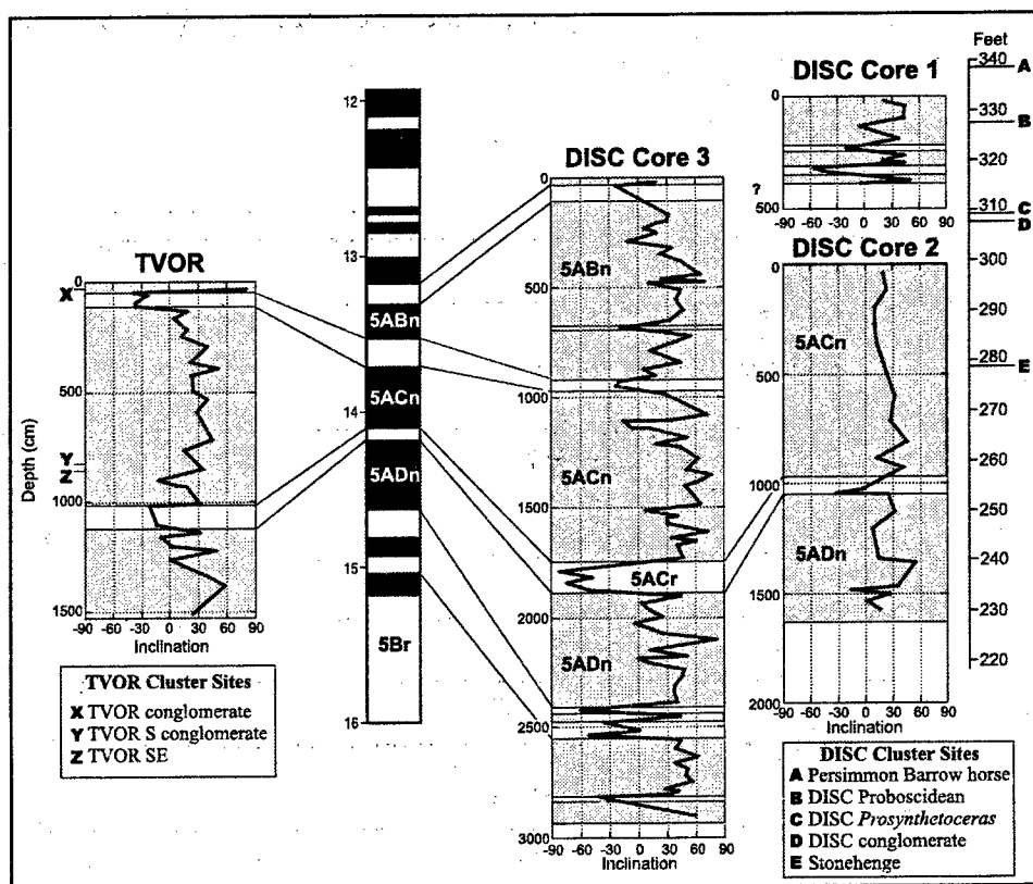
Figure 19. Correlation of polarity intervals between four cores at Fort Polk, Louisiana. Modified from Figure 33 of Schiebout et al. (2002) by the addition of new samples processed by Dr. Wulf Gose.
