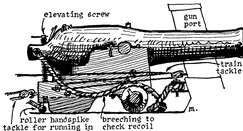
FIGURE 11—U. S. NAVY 9-INCH SHELL-GUN ON MARSILLY CARRIAGE (1866).
