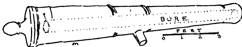
FIGURE 27—SPANISH 24-POUNDER CAST-IRON GUN (1693). Note the modern lines of this cannon, with its flat breech and slight muzzle swell.
