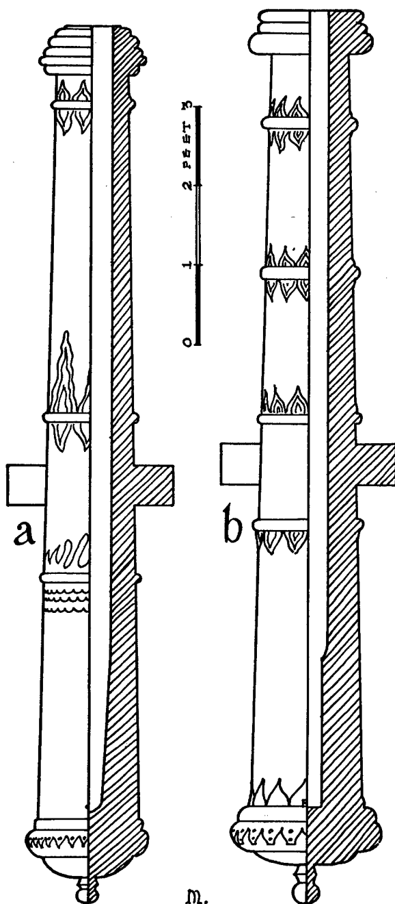
FIGURE 25—SIXTEENTH CENTURY CHAMBERED CANNON. a—"Bell-chambered" demicannon. b—Chambered demicannon.
