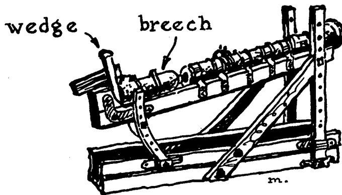
FIGURE 5—FIFTEENTH-CENTURY BREECHLOADER.
