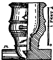
FIGURE 43—SPANISH 16-INCH PEDRERO (1788). This mortar fired baskets of stones.
