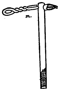
FIGURE 19—FRICTION PRIMER.
