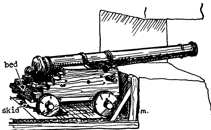
FIGURE 7—FRENCH GARRISON GUN (1650-1700). The gun is on a sloping wooden platform at the embrasure. Note the heavy bed on which the checks of the carriage rest and the built-in skid under the center of the rear axletree.
