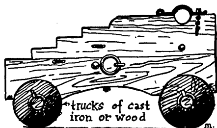
FIGURE 30—ENGLISH GARRISON CARRIAGE (1756). By substituting wooden wheels for the cast-iron ones, this carriage became a standard naval gun carriage.
