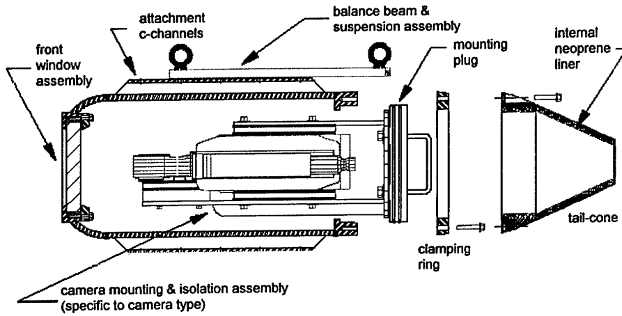
Figure 7. The shock resistant UNDEX camera housing. Schematic taken from [6]
