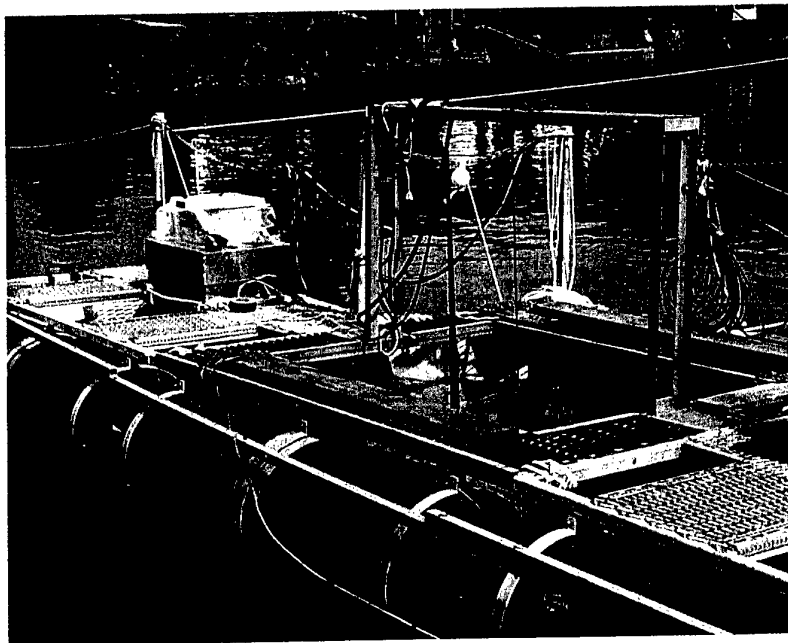
Figure 2. The imaging facility. The top view shows the overall arrangement of modular surface platforms together with the attendant filter 'barge' below and transport rig at right. The bottom view shows a close-up of the specialised camera handling platform. Note the foam filled rubber buoyancy tubes.
