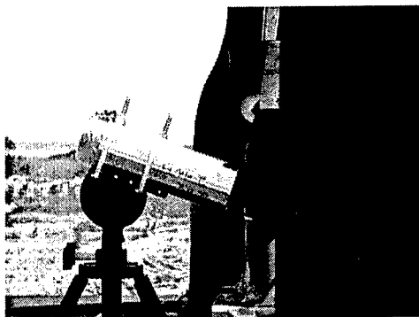
a. Predetonation setup of 81-mm mortar with MCD tool
