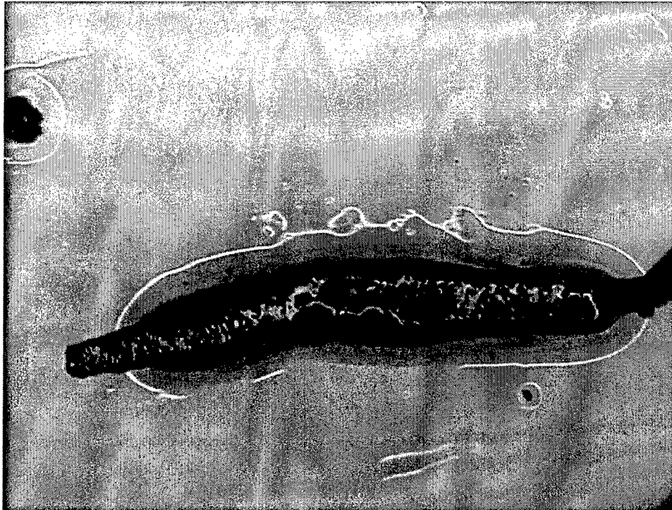
Figure 1-1. Development of red coloration in a fibrous particle of nitrocellulose when treated with a reagent that reacts with 2,4DNT. Particle was recovered near a firing point at Fort Richardson, Alaska
