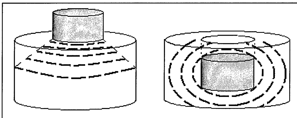
Figure 4-11. Detonation wave propagation in surrogate (left) vs. real (right) PMA-2
