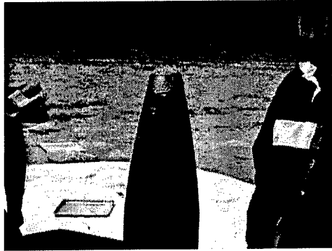
a. Predetonation setup of 155-mm projectile with C4 in fuze well
