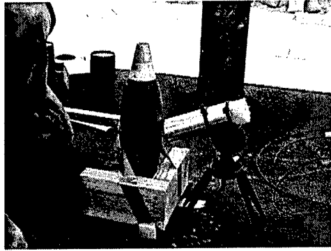
a. Predetonation setup of 81-mm mortar and MCD tool
