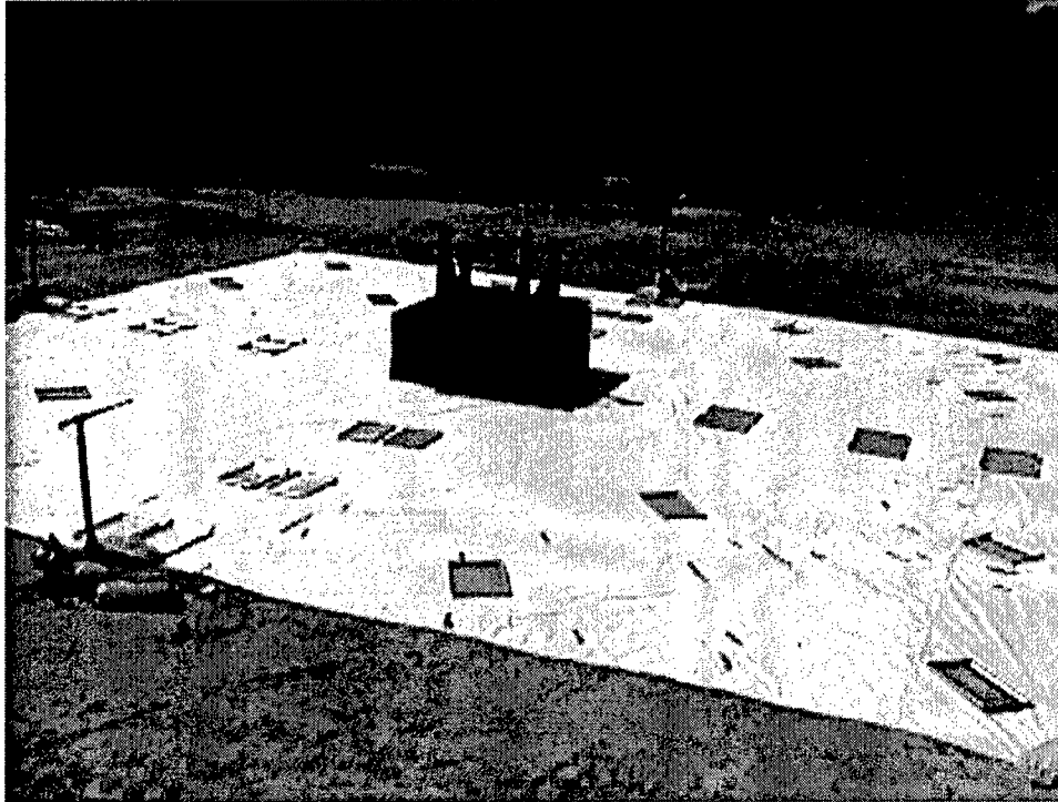
Figure 5-1. Setup of the system with witness plates, tarp, and pressure gauges
