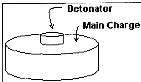
Figure 4-10. PMA-2 landmine schematic
