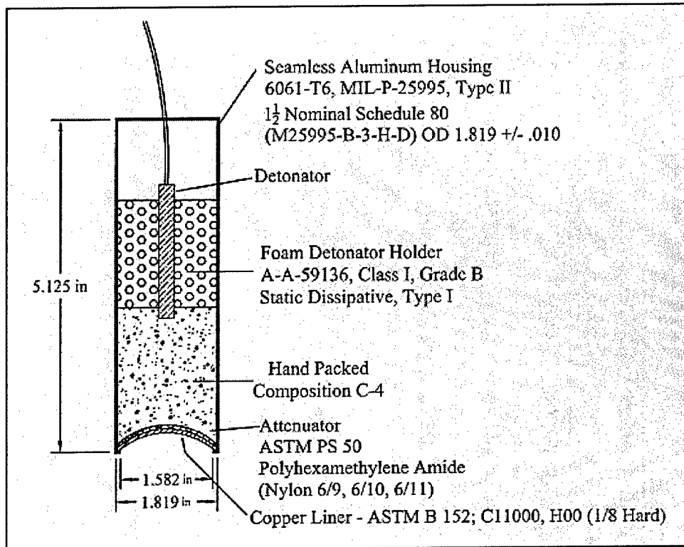
Figure 5-2. Assembly drawing of the MCD tool with material callouts (www.astm.org)
