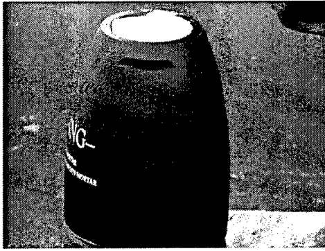
a. Predetonation setup of 81-mm mortar with C4 in fuze well
