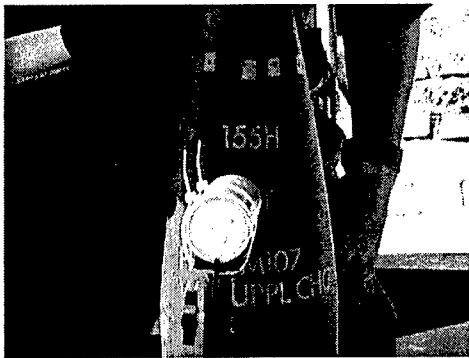
a. Predetonation setup of 155-mm projectile with MCD tool
