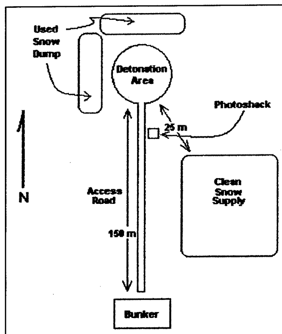
Figure 4-2. Site setup
