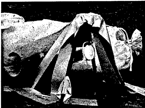
a. Setup of the MCD tool against 1/2-in. piece of fragment against sandbag
