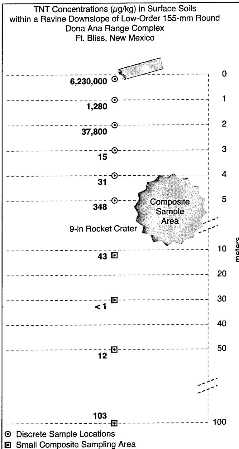
Figure 2-17. TNT concentrations ( \mu\text{g}/\text{kg}^{-1} ) for surface soil samples collected in a ravine downslope from a low-order 155-mm round at the artillery impact area at Dona Ana Range, Fort Bliss, New Mexico
