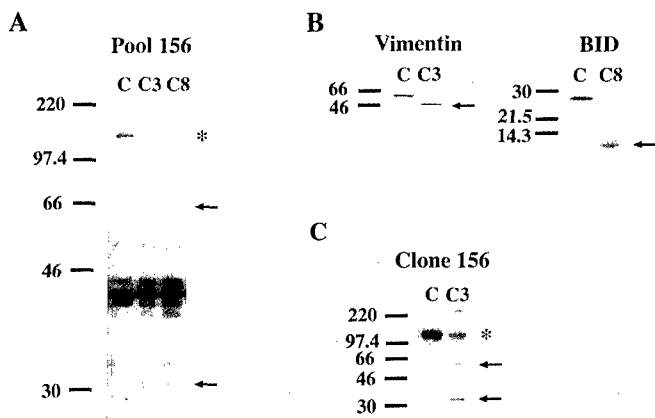
FIG. 1. Isolation of RAD21 as a caspase-3 substrate in vitro by small pool expression cloning. A , ^{35}\text{S} -labeled protein pool 156 contains a 125-kDa protein (indicated by the asterisk) that is specifically proteolyzed into two products of ~65 and 32 kDa (indicated by arrows) by caspase-3 (C3) but not by control (C) buffer or caspase-8 (C8). B , selective proteolysis of ^{35}\text{S} -labeled vimentin by caspase-3 (C3) and ^{35}\text{S} -labeled BID by caspase-8 (C8) into their signature cleavage fragments (indicated by arrows). C , identification of a single cDNA from pool 156 that encodes a 125-kDa protein (indicated by the asterisk) that is cleaved by caspase-3 (C3) into the appropriately sized products (indicated by arrows). cDNA pool 156 was subdivided, and the corresponding ^{35}\text{S} -labeled protein pools were re-examined as above until a single cDNA encoding the caspase-3 substrate was isolated. Sequencing of this clone revealed that it is a partial human rad21 cDNA. Small pool expression cloning, cleavage reactions, and analysis of proteolytic products were performed as detailed under "Experimental Procedures" and elsewhere (11–13). The molecular mass of markers in kDa is indicated at the left of each panel.
