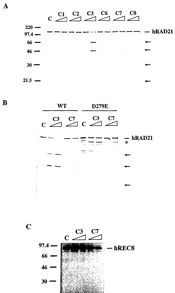
FIG. 2. Human RAD21 is specifically cleaved by caspases-3 and -7 at multiple sites, including Asp 279 , to yield several proteolytic products in vitro . A , ^{35}\text{S} -labeled full-length human RAD21 was incubated with control (C) buffer or 2.5 or 25 ng of caspase-1, -2, -3, -6, -7, or -8 (C1–C8) for 1 h at 37 °C, and the reaction products were resolved by SDS-PAGE. The cleavage fragments are indicated by arrows. B , RAD21 mutant D279E is resistant to proteolysis at Asp 279 by caspases-3 and -7 in vitro . ^{35}\text{S} -labeled WT or mutant D279E RAD21 were incubated with control (C) buffer or 10 or 25 ng of caspases-3 (C3) or -7 (C7) for 1 h at 37 °C. WT RAD21, but not the D279E mutant, was proteolyzed into major fragments of 65 and 48 kDa (indicated by arrows). The D279E mutant was cleaved into a single larger product (indicated by the asterisk) that was not observed when WT RAD21 was incubated with caspases-3 or -7 in vitro . C , Human REC8, a homologue of RAD21, is not cleaved by caspases-3 or -7 in vitro . ^{35}\text{S} -labeled human REC8 was incubated with control (C) buffer or 2.5 or 25 ng of caspase-3 (C3) or caspase-7 (C7) for 1 h at 37 °C. The molecular mass of markers in kDa is indicated at the left of each panel.
