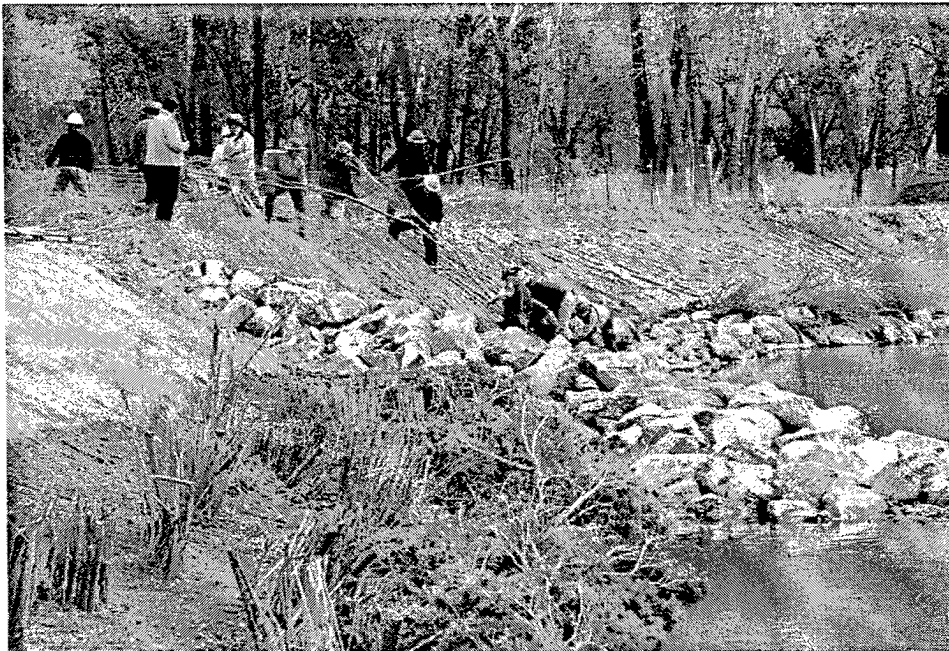
Figure 4. Incorporating irregular alignments, features such as spurs, and other habitat measures into a revetment can significantly improve habitat benefits
