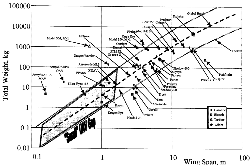
FIGURE E-1: UAV WINGSPAN VS. WEIGHT.
