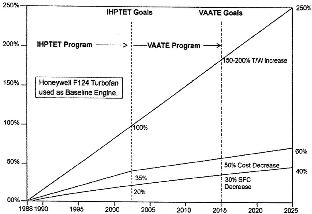
FIGURE D-6: IHPTET AND VAATE PROGRAM GOALS AND TRENDS.
