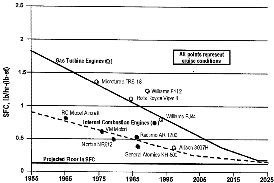
FIGURE 4.1-1: SPECIFIC FUEL CONSUMPTION TRENDS.
