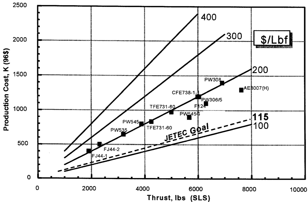
FIGURE A-2: JETEC COST GOAL IN COMPARISON TO EXISTING SYSTEMS. CLEARLY, INNOVATIVE, LOW-COST DESIGN AND MANUFACTURING TECHNIQUES MUST BE DEVELOPED TO MEET THIS GOAL.
