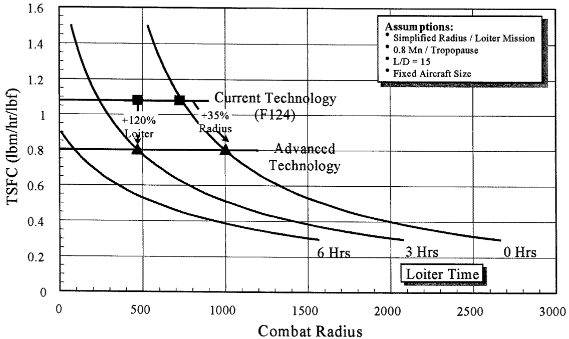
FIGURE A-1: THE PERFORMANCE PAYOFF OF A NOTIONAL COMBAT UAV UTILIZING TECHNOLOGIES FROM THE SUCCESSFUL DEMONSTRATION THE JETEC PHASE III GOALS.
