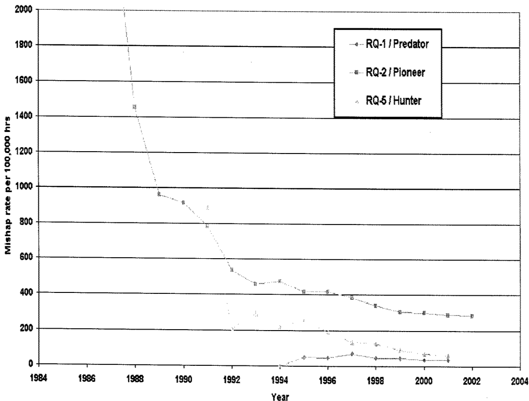
FIGURE G-2: US MILITARY UAV MISHAP RATES, 1986-2001
