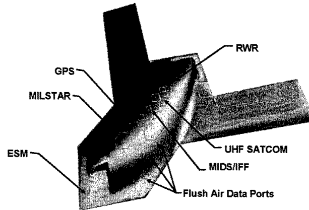
FIGURE I-9: UCAV APERTURES.
