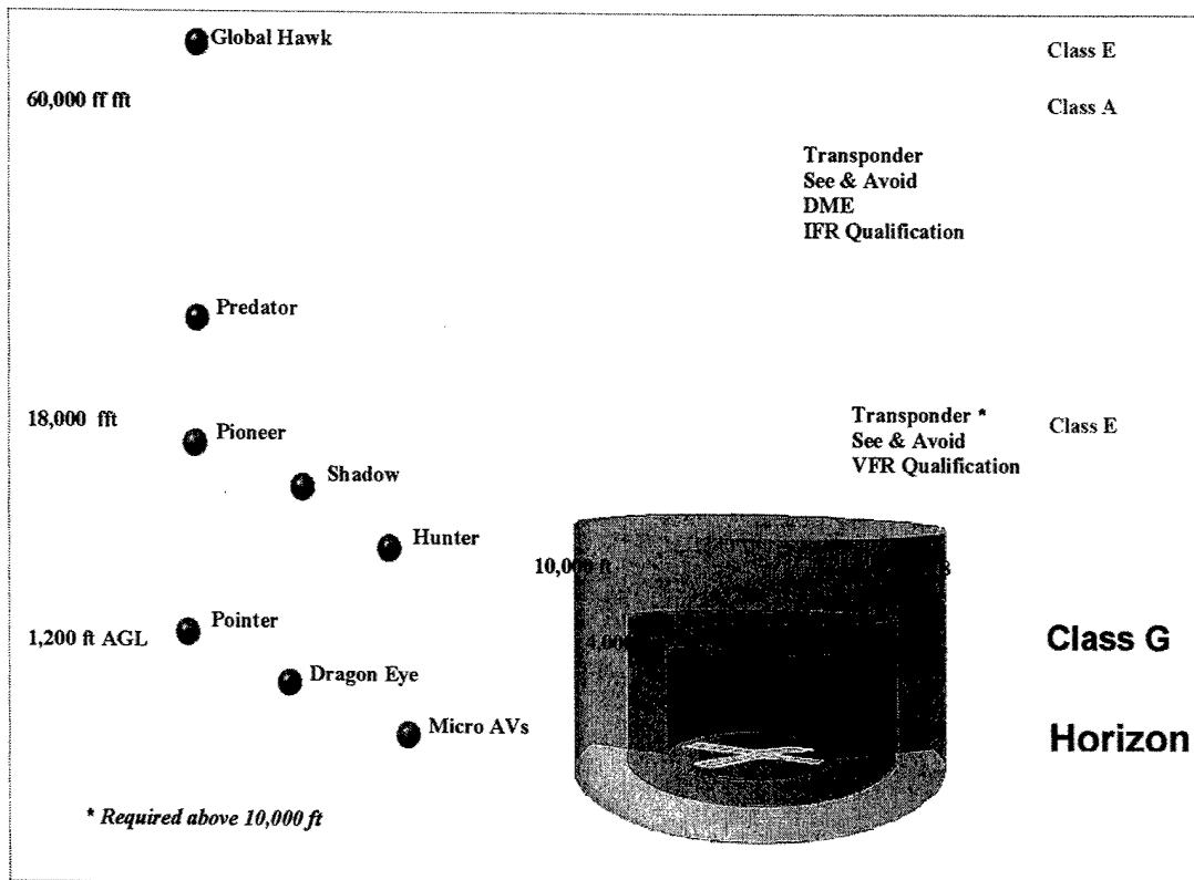
FIGURE G-3: UAVS AND AIRSPACE CLASSES OF THE NATIONAL AIRSPACE SYSTEM.
