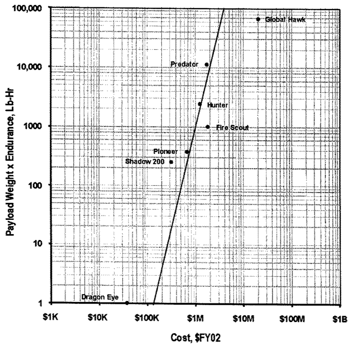
FIGURE 4.1-5: UAV PERFORMANCE METRIC: ENDURANCE V. COST.
