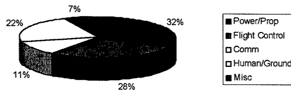
FIGURE J-3: AVERAGE SOURCES OF SYSTEM FAILURES FOR IAI UAV FLEET (BASED ON 100,000 HOURS)
