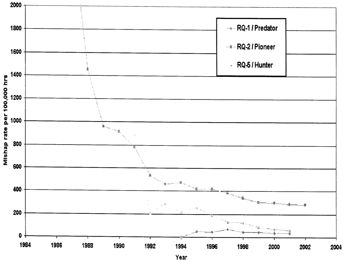
FIGURE 5.2-1: UAV MISHAP RATE TRENDS.
