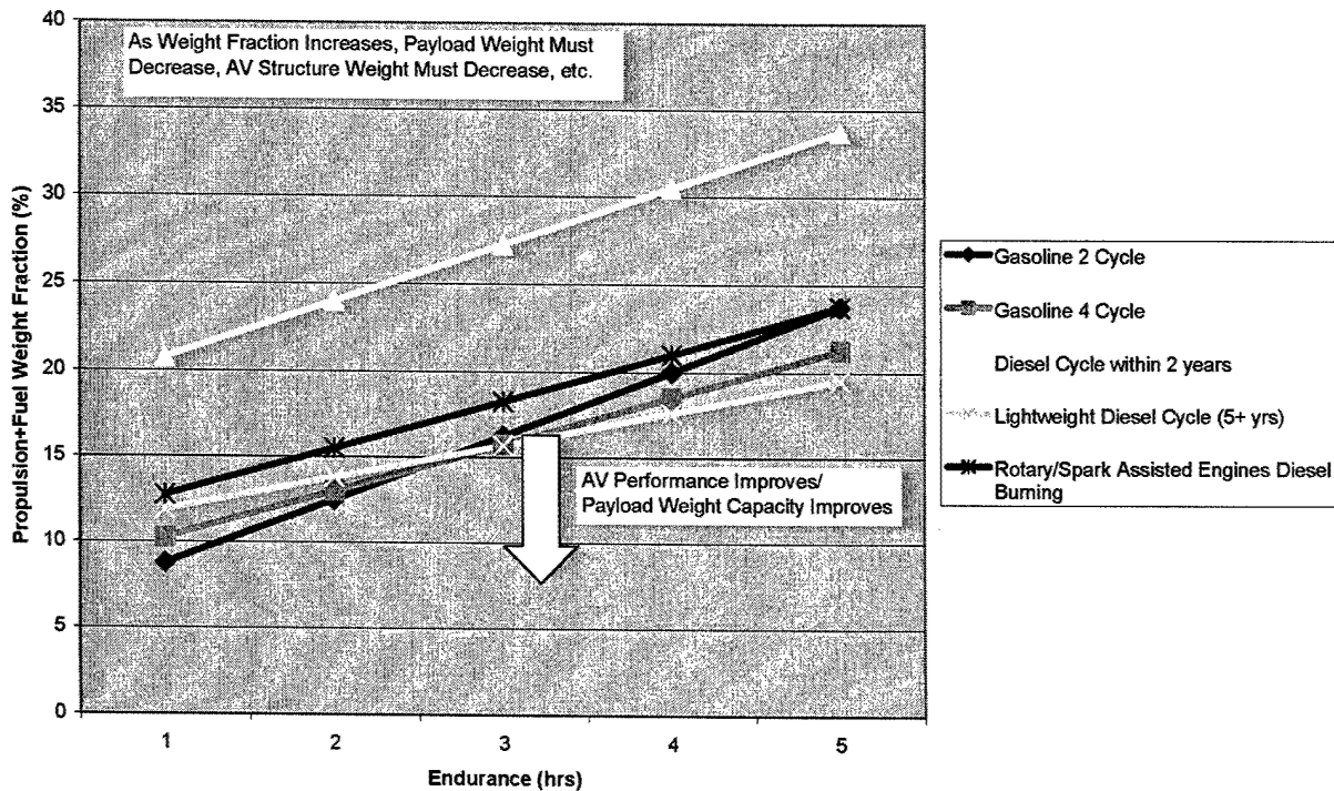
FIGURE A-3: ENGINE EFFECTS ON TAKEOFF GROSS WEIGHT FOR A DESIRED MISSION ENDURANCE
