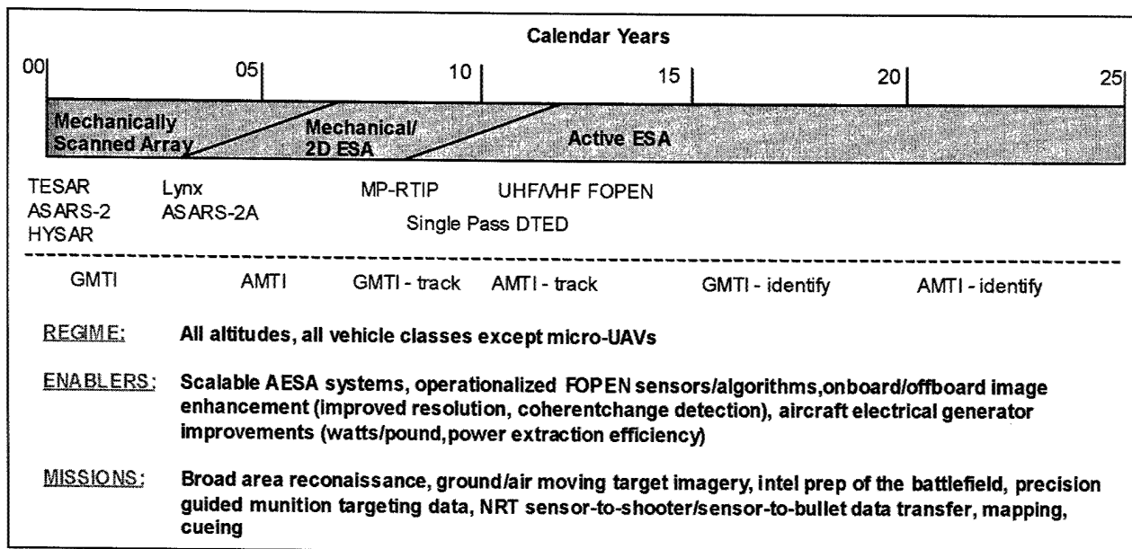
FIGURE 4.2-4: RADAR IMAGER SENSOR TECHNOLOGY FORECAST.
