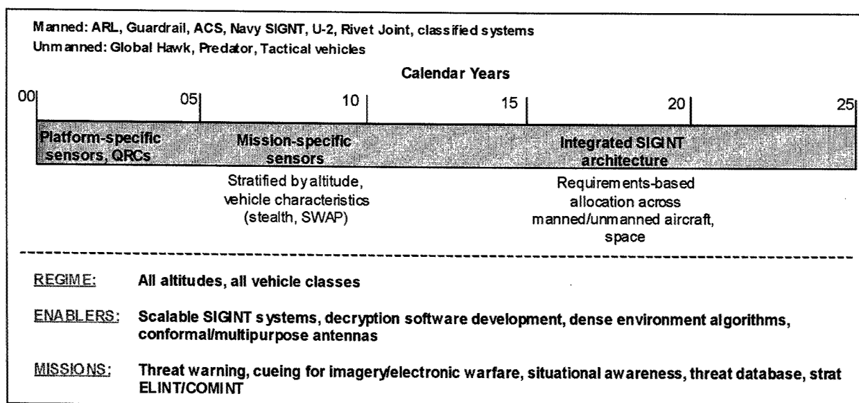
FIGURE 4.2-5: SIGINT SENSOR TECHNOLOGY FORECAST.
