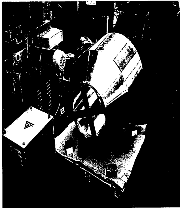
Figure B4. Aluminum Explosive Housing/Explosive Loading Fixture
