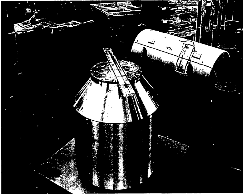
Figure 10. Assembled CSC
