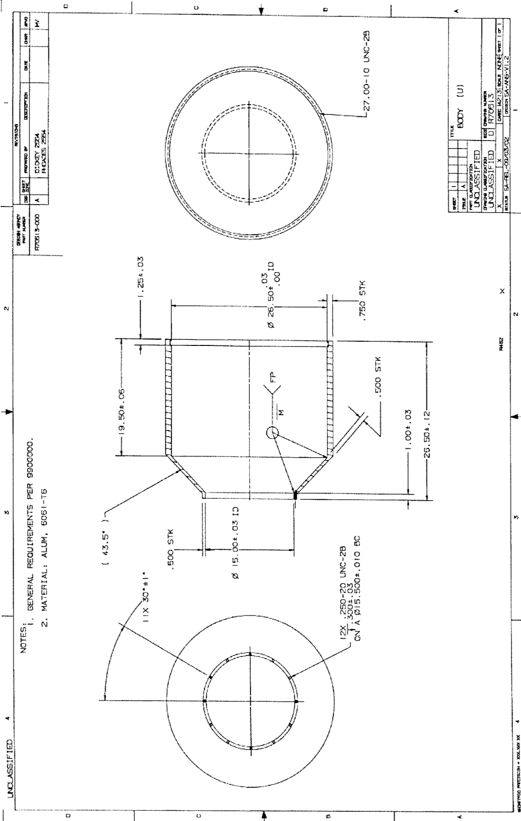
Figure A3. Explosive Housing
