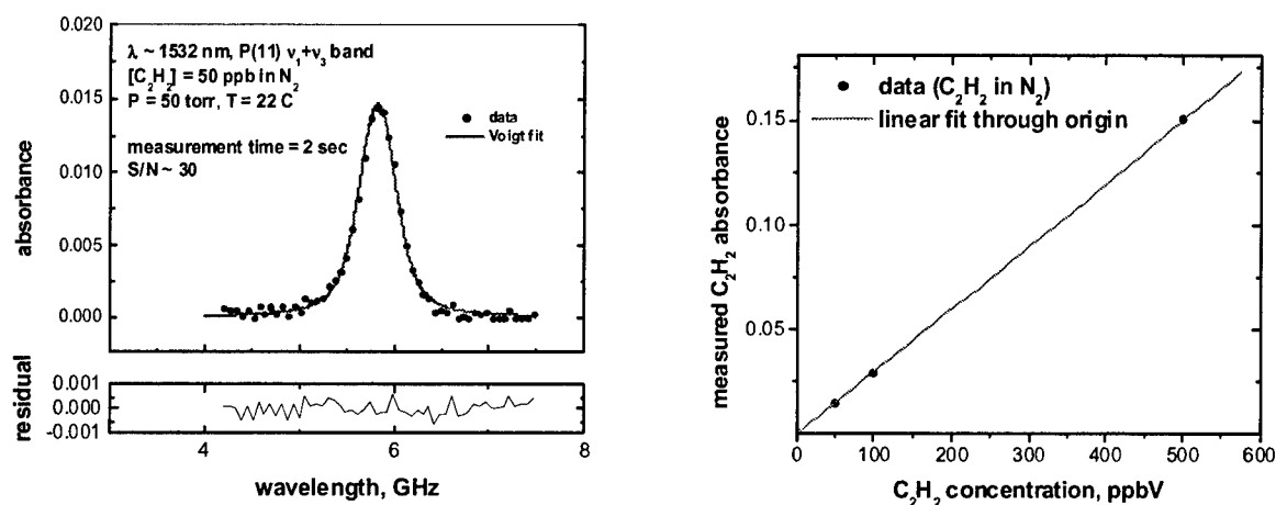
Figure 2. (Left) Measurements of C_2H_2 absorption [P(11) line, v_1+v_3 band]] near 1532 nm obtained using off-axis ICOS. (right) Comparison of measured C_2H_2 absorption with various mixture fractions of C_2H_2 in N_2 .
