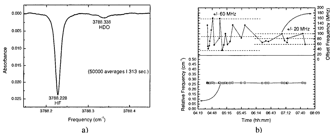
Fig.2: a) Direct absorption spectra of HF and HDO at 2.64 \text{ }\mu\text{m} ( p<10 \text{ Torr} ). The residual peak-to-peak baseline noise is <0.01\% . b) Spectroscopic stability in units of \text{cm}^{-1} and MHz over a 200-minute time period. The peak fit precisions were better than \pm 4 \text{ MHz} and are represented as solid squares in the upper graph 2.b).
