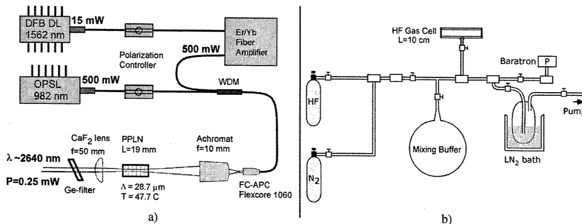
Fig.1: a) Schematic of difference frequency generation laser source at 2.64\ \mu\text{m} . OPSEL, optically pumped semiconductor laser; DFB DL, distributed feedback diode laser; WDM, wavelength division multiplexer; FC-APC, fiber coupler – angled polished connector; b) Schematic of HF gas filling line. LN 2 , liquid nitrogen.
