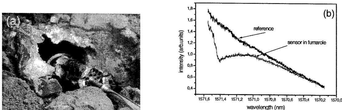
Figure 3: (a) In-situ application of the evanescent-field laser sensor at the volcano site "Solfatara" (Italy). (b) Wavelength scan for the detection of \text{H}_2\text{S} directly in the volcano fumerole.
