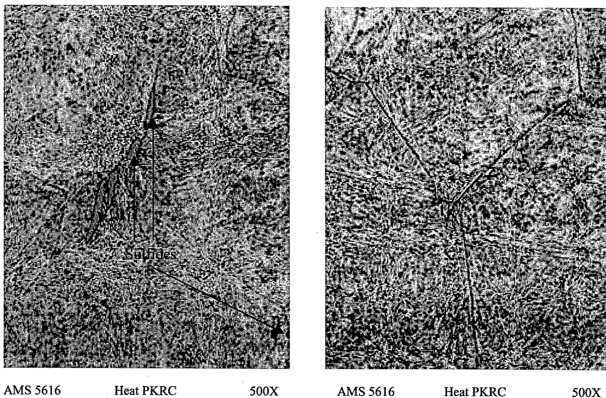
FIGURE 11. TYPICAL MICROSTRUCTURE OF AMS 5616 BARSTOCK HEAT PKRC AFTER ONE (LEFT) AND EIGHT (RIGHT) STRESS RELIEF CYCLES AT 1050°F (2 HRS) (Note the presence of sulfides in the grain boundaries and more clearly delineated grain boundaries (right) indicative of a sensitized condition with grain boundaries filled with carbides and other particles, compared to the cleaner structure of rolled ring material (heat ZCESS) illustrated in figure 7.)
