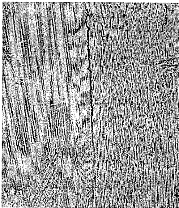
Outer Center Ring Repair 50X
