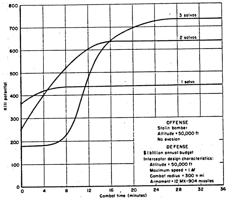
Fig. 40—Effect of combat time and number of salvos on interceptor effectiveness
