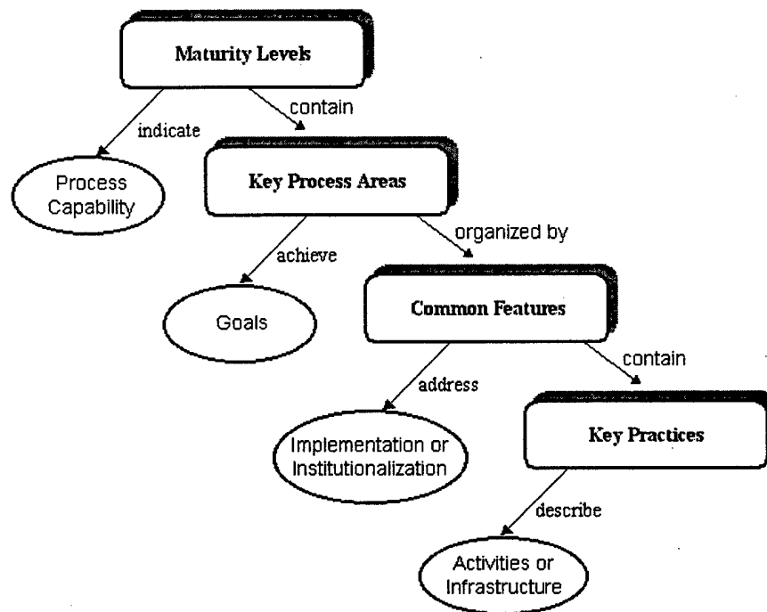
Figure 12: The Structure of the Capability Maturity Model
