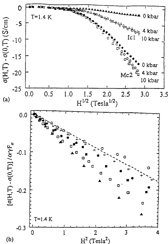
Fig. 2.40 (a) High field magnetoconductance of PPy-PF 6 samples plotted as a function of H^{1/2} at T = 1.4 K and P = 4 kbar and 10 kbar. (b) The low field magnetoconductance normalized by \alpha\gamma F_\sigma plotted as a function of H^2 for sample M2 at P = 9 kbar (○), \rho_r = 1.33 ; Mc2 at P = 10 kbar (+), \rho_r = 1.54 ; M2 (●), \rho_r = 1.97 ; Mc2 (■), \rho_r = 3.2 ; Mc3 (■), \rho_r = 4.5 and Ic1 (▲), \rho_r = 12 . The dashed line is the theoretical estimate [44,45].
