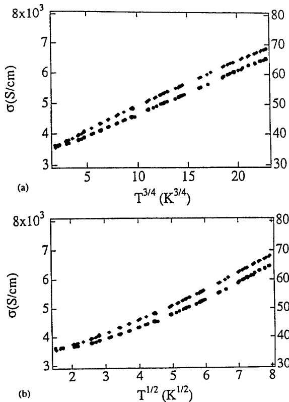
Fig. 2.18 (a) \sigma(T) vs. T^{3/4} for I-(CH) x and (b) conductivity vs. T^{1/2} for I-(CH) x (●) parallel to the chain axis; (◆) perpendicular to the chain axis.
