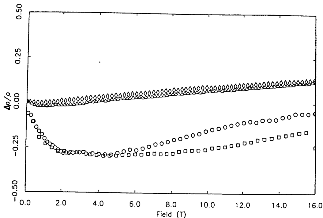
Fig. 2.42 Magnetoresistance ( \Delta\rho/\rho ) vs. H for PPy-PF 6 sample M1 at 20 mK (□), 70 mK (○), 370 mK (△), 500 mK (◇). (From Ref. 151.)
