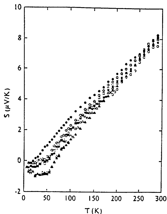
Fig. 2.63 S(T) vs. T of PANI-CSA/PMMA blends at various concentrations of PANI-CSA in PMMA: y = 100\% (●), 66.6% (◇), 33.3% (□), 9.09% (*), 4.76% (+), 2.43% (△), 1.24% (○).
