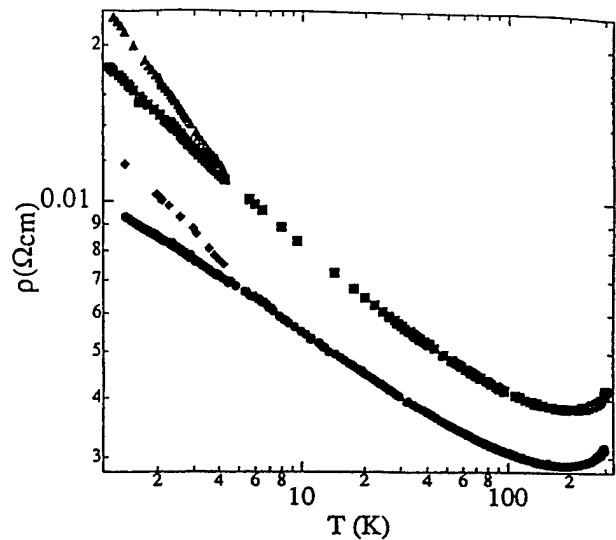
Fig. 2.6 Log-log plot of the \rho(T) vs. T for two PANI-CSA samples in the critical regime: H = 0 T (●) and H = 10 T (◆) for sample with \rho(T) \propto T^{-0.26} ; H = 0 T (■) and H = 8 T (▲) for sample with \rho(T) \propto T^{-0.36} .
