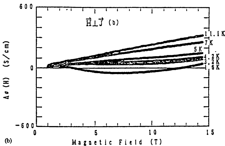
Fig. 2.25 Magnetoconductance versus H of I-(CH)_x ( \rho_r \approx 3.7 ) (a) for longitudinal field; (b) for transverse field. (From Ref. 127.)
