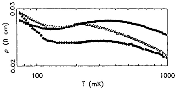
Fig. 2.30 Data of \rho(T) vs. T for PANI-CSA in the metallic regime at 0 T (●), 2 T (△), and 8 T (■). (From Ref. 151.)
