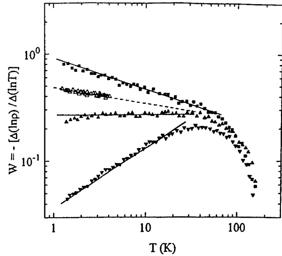
Fig. 2.5 Log-log plots of W vs. T for PANI-CSA in the metallic regime (▼); the critical regime at ambient pressure and H = 0 (▲) and at ambient pressure and H = 8 T (△); and the insulating regime (■). The lines are drawn to guide the eye.
