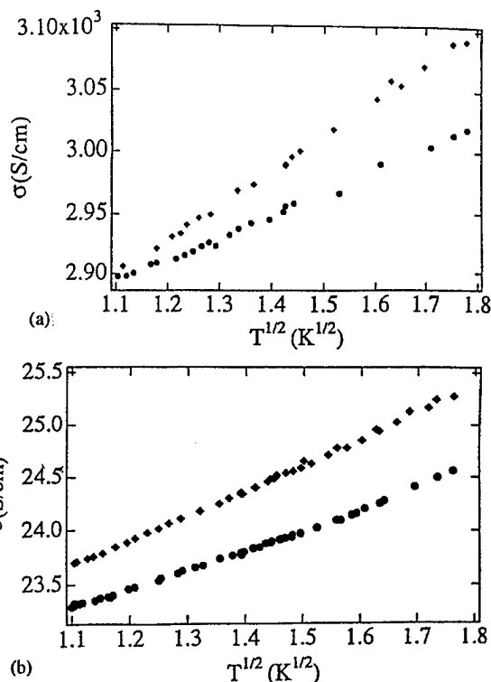
Fig. 2.22 Conductivity versus T^{1/2} for I-(CH)_x (a) parallel to the chain axis and (b) perpendicular to the chain axis ( \bullet ) at H = 0 and ( \blacklozenge ) at H = 8 T.
