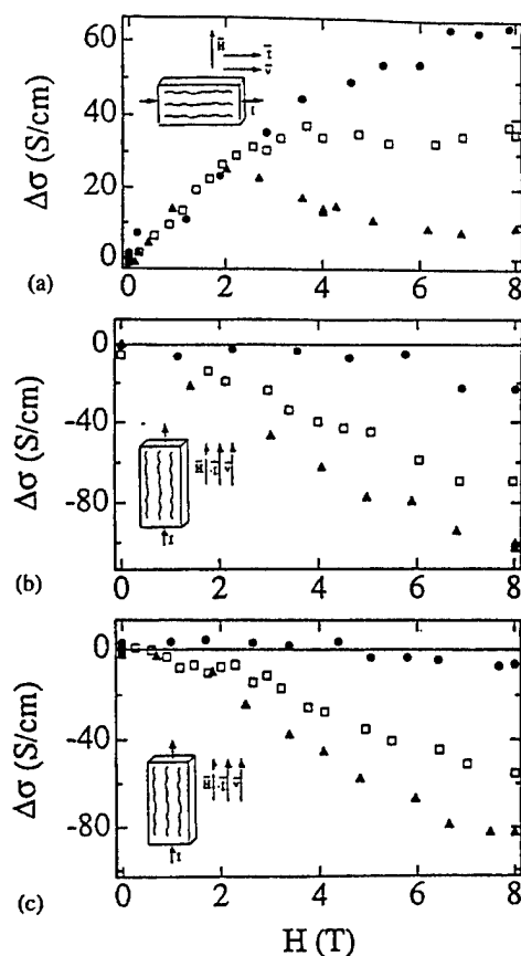
Fig. 2.23 Magnetoconductance versus H for \text{I}-(\text{CH})_x at 4.2 K ( \bullet ), 2 K ( \square ), and 1.2 K ( \blacktriangle ). The current is parallel to the chain axis. (a) The field is perpendicular (perpendicular) to the chain axis (current); (b) the field is parallel (parallel) to the chain axis (current) at ambient pressure; (c) the field is parallel (parallel) to the chain axis (current) at 8 kbar.
