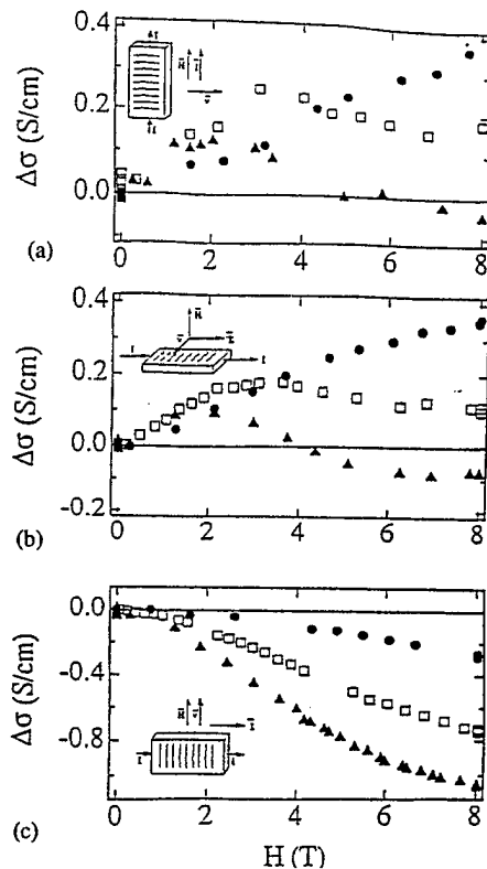
Fig. 2.24 Magnetoconductance versus H for I-(CH)_x at 4.2 K ( \bullet ), 2 K ( \square ), and 1.2 K ( \blacktriangle ). The current is perpendicular to the chain axis ( n ). (a) The field is perpendicular to the chain axis (parallel to the current); (b) the field is perpendicular to the chain axis and current; (c) the field is parallel to the chain axis. (perpendicular to the current).
