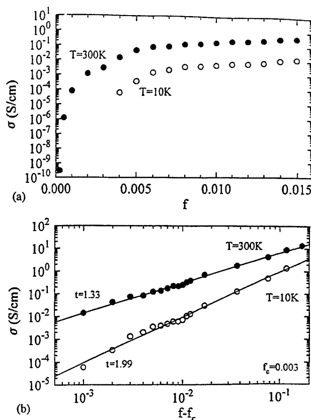
Fig. 2.55 (a) Conductivity ( \log_{10} scale) versus volume fraction ( f ) of PANI-CSA at 300 and 10 K. (b) \log_{10}\text{--}\log_{10} plot of \sigma vs. (f - f_c) at 300 K (●) and 10 K (○), where f_c = 0.003 . The solid line through the points corresponds to a slope ( t ) of 1.99 at 10 K and 1.33 at 300 K, respectively.
