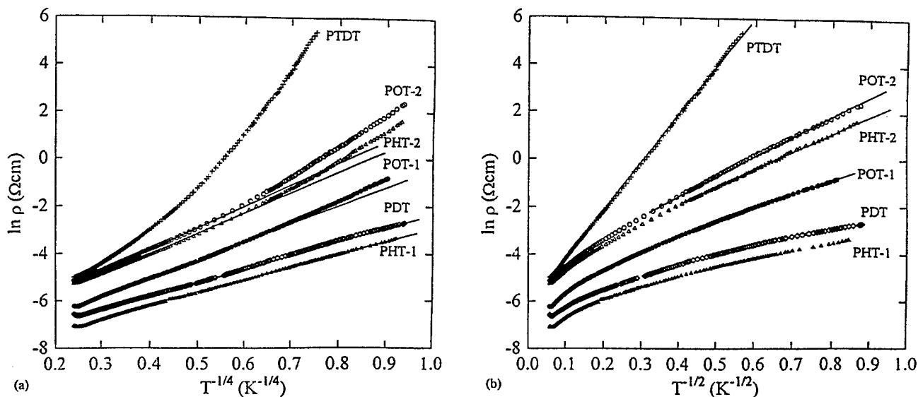
Fig. 2.46 (a) \ln \rho vs. T^{-1/4} for iodine-doped PAT samples. Solid lines represent linear fit regions. (b) \ln \rho vs. T^{-1/2} for the same data. Solid lines represent linear fit regions. Symbols are described in Table 2.6.
