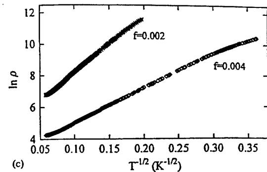
Fig. 2.58 Natural log of resistivity versus T^{-\gamma} (a) \gamma \approx 2/3 for f = 0.12, 0.08, 0.04 , and 0.02 ; (b) \gamma \approx 1 for f = 0.012, 0.008 , and 0.006 ; (c) \gamma = 1/2 for f = 0.004 and 0.002 .
