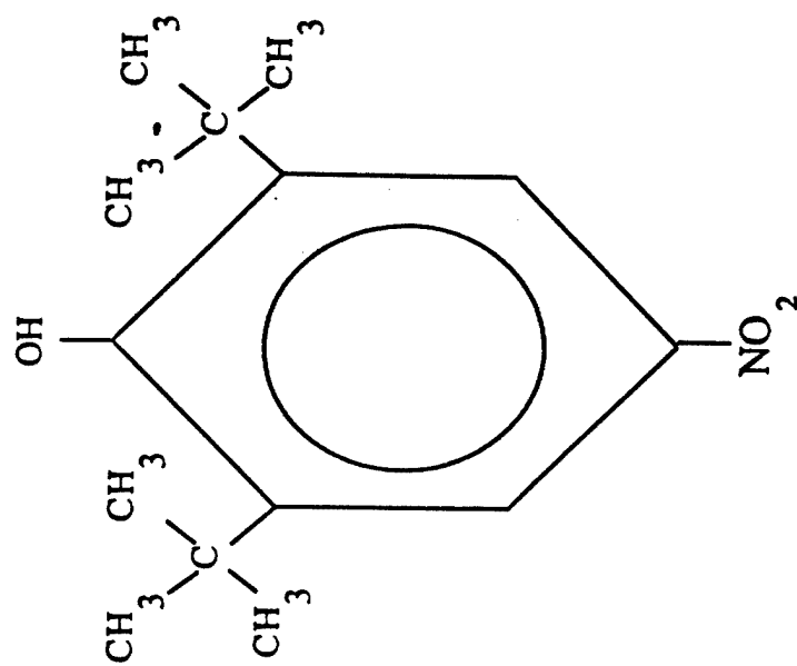
2, 6 di-t-butyl-4-nitrophenol
