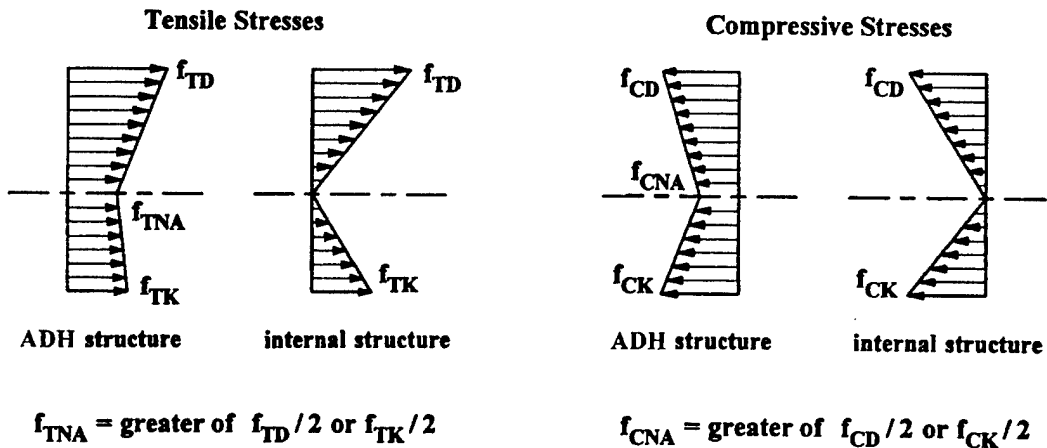
Figure 4. Primary Longitudinal Design Stress
