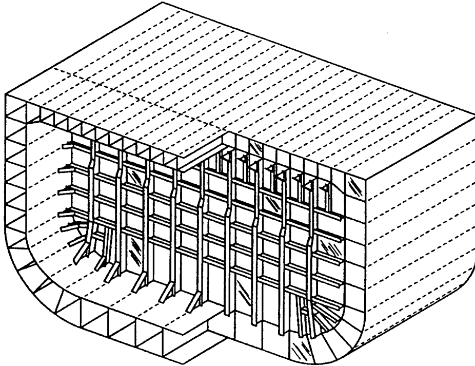
Figure 12. Advanced Double Hull Transverse Bulkhead Design Configuration
