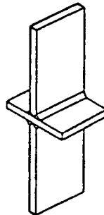
(E) Full penetration, load carrying filled welds. Discontinuous member loaded.
