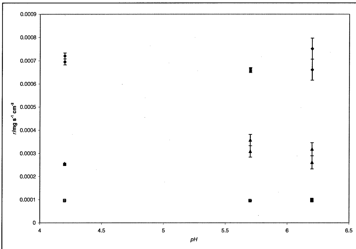
Figure 36. Comparison of explosive dissolution rates at three pH values: \blacklozenge TNT, \blacktriangle HMX, \blacksquare RDX. Vertical bars are standard deviations from the mean
