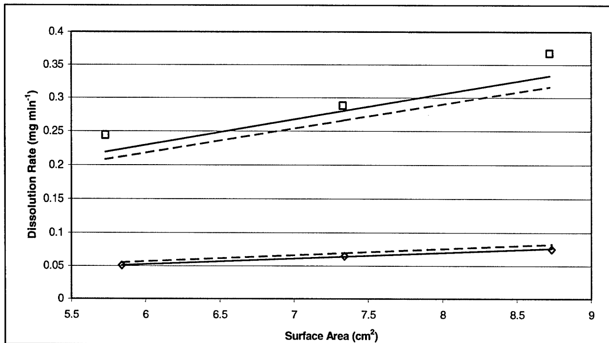
Figure 31. Rate comparisons of TNT study data ( \square = 30 °C data, \diamond = 10 °C data) to multiple regression-multiple variable regression line (—) and the Levins and Glastonbury (1972a) regression line (---)
