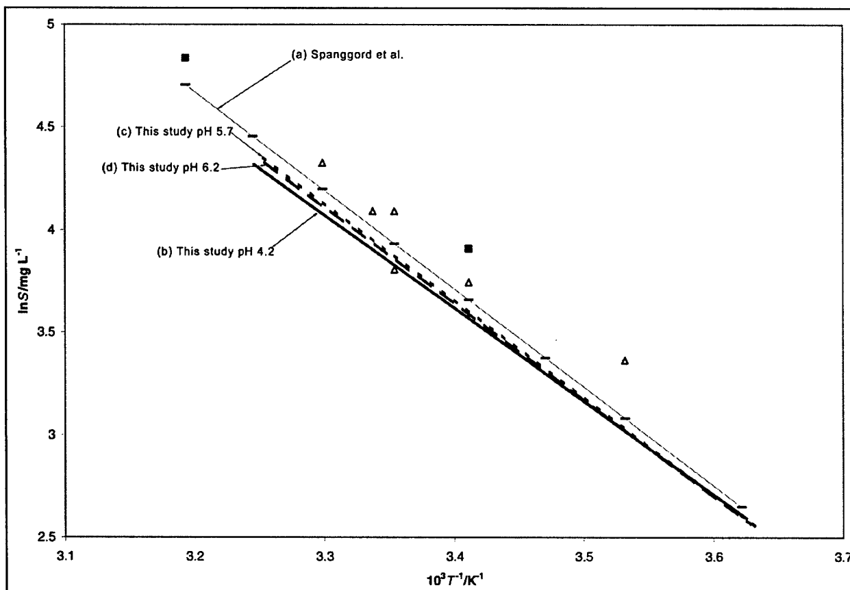
Figure 33. Comparison of RDX solubility literature to this study. (a) Spangord et al. (1983); ■ Gibbs and Popolato (1980); Δ Townsend and Meyers (1996); (b) this study pH 4.2 [ \ln(S/\text{mg L}^{-1}) = 19.087 - 4,549.1 K/T , R^2 = 0.987 ]; (c) this study pH 5.7 [ \ln(S/\text{mg L}^{-1}) = 19.718 - 4,727.8 K/T , R^2 = 0.995 ]; (d) this study pH 6.2 [ \ln(S/\text{mg L}^{-1}) = 19.818 - 4,753.2 K/T , R^2 = 0.995 ]
