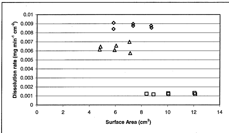
Figure 28. Surface area comparison of explosives at 150 rpm and 10°C ( \diamond = TNT, \square = RDX, \Delta = HMX)
